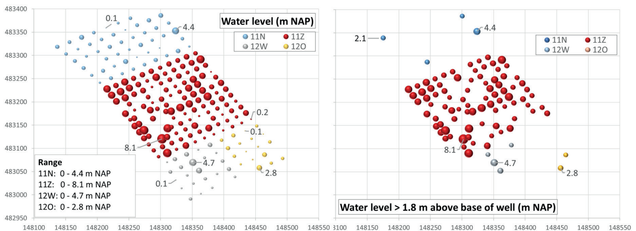
FIGURE 3: Water levels in compartments 11N, 11Z, 12W and 12O normalized to m +NAP (Normaal Amsterdams Peil, Amsterdam Ordinance Datum) March 2020 (left), levels exceeding the height of the filter screen (right). The size of the symbol is indicative of water level. Coordinates given in EPSG:28992 (Amersfoort datum).
