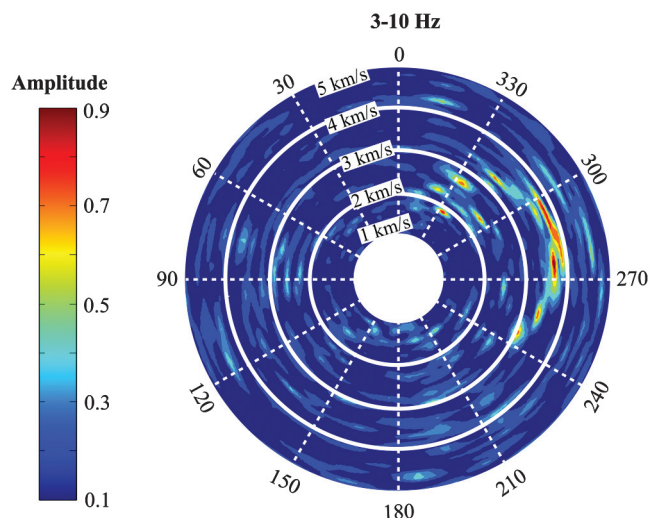
Figure 4. Directional beam-forming analysis for recorded noise from February 2015 where the maximum beam power of each hourly panel and its apparent velocity and azimuth are shown for the frequency range of 3–10 Hz. The north direction has an azimuth of 0^\circ . The azimuth increases to the west (i.e., counterclockwise).
