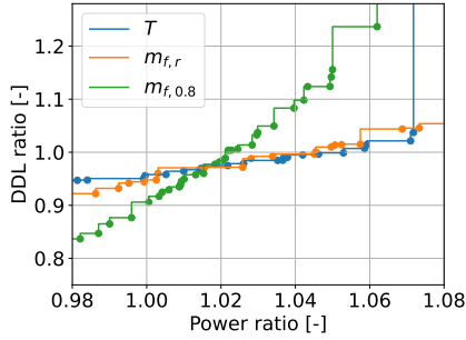
Figure 9. Pareto front for the downwind winglet optimizations
