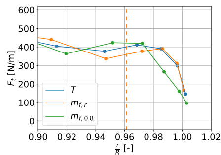
Figure 14. Tangential loads for three optimized upwind winglet
