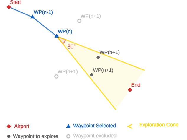
Fig. 3. The exploration cone limits the number of nodes to explore.
