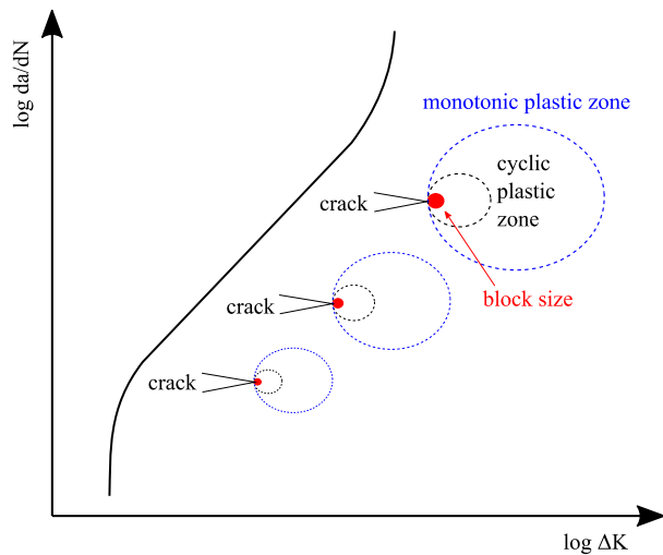
Fig. 21. Schematic illustration of monotonic and cyclic plastic zone and block size during FCG test.
