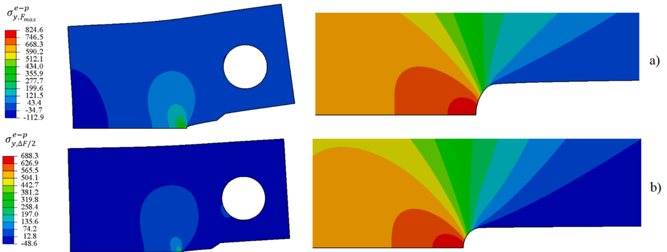
Fig. 13. Elastoplastic stress field (in MPa) for crack length a = 18.67\text{mm} and R_\sigma = 0.1 : a) at maximum load F = F_{max} ; b) at half of range load value F = \Delta F/2 .
