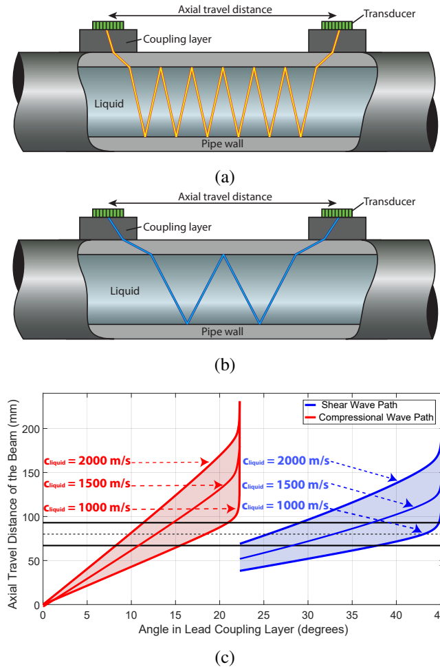
Figure 6: Travel path of an acoustic beam during clamp-on ultrasonic flow measurements using (a) compressional, and (b) shear waves in the pipe wall. (c) Axial travel distance of the beam (equal to the axial transducer separation) versus the beam angle in the coupling layer, for a pipe with an inner diameter of 40 mm. The black dashed line represents the physical location of the center of the receiver transducer array (80 mm), and the black solid lines give the boundaries of its aperture in the axial direction.
