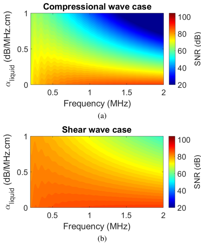
Figure 3: Computed SNR of the designed transducer array, versus frequency and attenuation coefficient of the liquid. (a) Compressional waves in the pipe wall and six bounces (v-shapes) of the acoustic beam within the pipe. (b) Shear waves in the pipe wall and two bounces (v-shapes) of the acoustic beam within the pipe.
