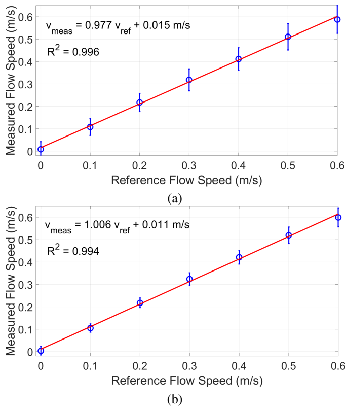
Figure 13: Measured versus reference flow speed of water for the acoustic beam paths of (a) Fig. 6a and (b) Fig. 6b. Vertical bars indicate median absolute deviations.
