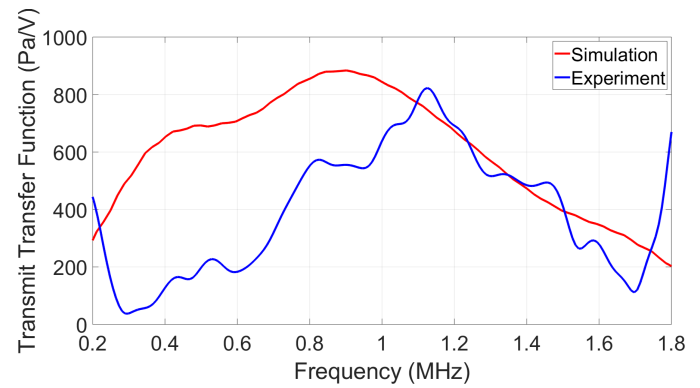
Figure 8: Measured and simulated transmit transfer function, in water, of the prototype linear transducer array of Fig. 7.
