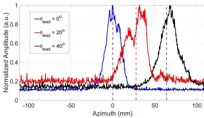
Figure 9: Measured linear scans of the amplitude of the acoustic wavefield in water, generated by the transducer array of Fig. 7 for three different beam steering angles in lead. The dashed vertical lines indicate the theoretical expected position of the peak pressures for the theoretical sound speeds involved.
