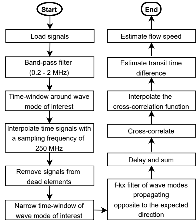
Figure 11: Signal processing sequence applied to the measured signals from the flow sensor of Fig. 10.
