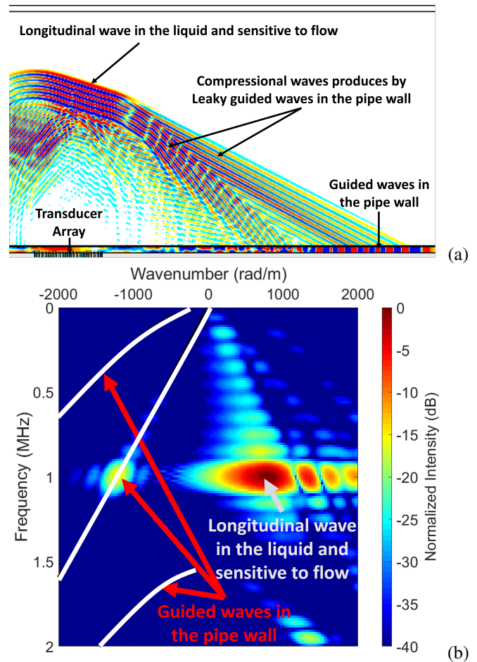
Figure 5: (a) Finite Element simulation of the acoustic field generated by a transducer array with beam steering, located on the bottom side of a 1 mm-thick stainless steel pipe with an inner diameter of 40 mm and filled with a fluid with c_{\text{liquid}} = 1500 m/s and \alpha = 1 dB/MHz.cm. (b) Magnitude in the wavenumber-frequency domain of the narrow-banded time signals recorded along the bottom pipe wall (i.e. along the same surface on which the array is located) of the geometry in (a). The guided waves in the pipe wall have approximately 20 dB lower amplitude relative to the compressional wave that is refracted from the flow. The white lines represent the theoretical dispersion curves of the guided waves in the pipe wall.
