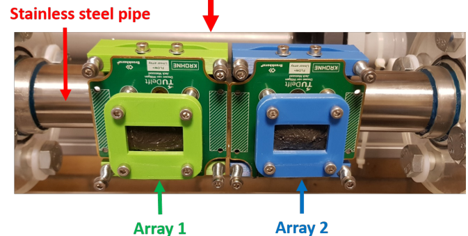
Figure 10: Custom-made flow loop to perform clamp-on ultrasonic flow measurements with our fabricated prototype arrays. The red oval indicates the location of the flow sensor with the two linear arrays (top figure). Gravity was used to drive flow from left to right through the stainless steel pipe section on which the arrays were installed (bottom figure). The custom-made 3D-printed green and blue frames were designed with a system of screws and springs to achieve mechanical coupling of the backing with the PCB (front screws), and of the lead coupling piece (not visible here) with the pipe wall (back screws).
