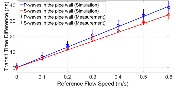
Figure 12: Theoretical transit time difference (solid lines) and measured transit time difference (circles) between upstream and downstream signals, versus flow speed, for the scenarios of Fig. 6a (blue) and Fig. 6b (red). Vertical bars indicate median absolute deviations.
