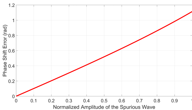
Figure 4: Nonlinear phase-shift error induced by spurious signals, versus the normalized amplitudes of these spurious signals. Amplitude is normalized to the maximum amplitude of the ‘clean’ upstream and downstream signals.
