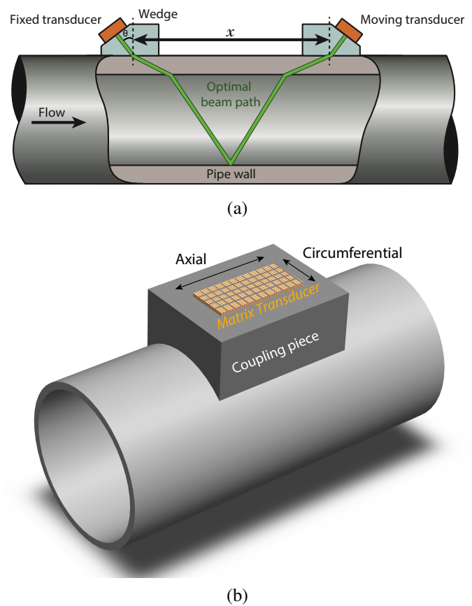
Figure 1: (a) Sketch of a conventional clamp-on ultrasonic flow meter. Upon installation, one single-element transducer is manually moved along the pipe wall to find the optimal distance x , which depends on the properties and geometry of the pipe wall, and on the sound speed of the liquid. The green line represents the path of the flow-sensitive wave. Here the wave bounces only once inside the pipe. For clarity, the travel paths of other waves are not shown. (b) Concept of a matrix transducer array for clamp-on ultrasonic flow metering, with array elements along the axial and the circumferential direction.
