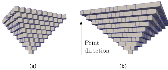
Fig. 5. The printable cone (the largest printable volume, starting from one element) using the original implementation [8], with a 5-element (a) or 9-element support (b).
