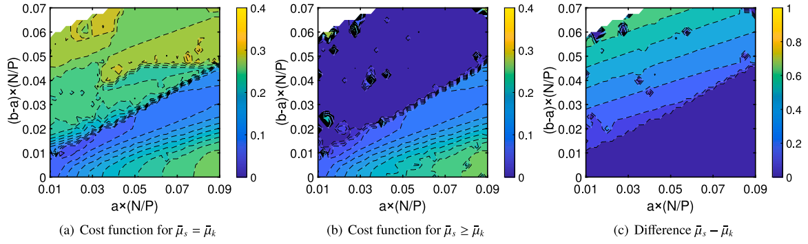
Fig. 19. Cost function obtained for optimal values of \bar{\mu}_k and \bar{\mu}_s of the Amontons–Coulomb friction model for r = 0.1 and \bar{\mu}_* = 0.2 (more than two stops stick-slip motion with the Dieterich–Ruina law), considering \bar{\mu}_s = \bar{\mu}_k (subfigure (a)) or \bar{\mu}_s \geq \bar{\mu}_k (subfigure (b)). The difference between the optimal values of \bar{\mu}_k and \bar{\mu}_s is shown in (subfigure (c)).
