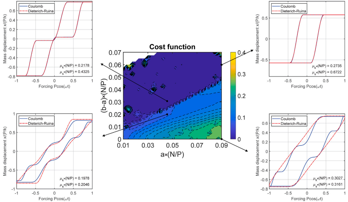
Fig. 20. Cost function obtained for optimal values of \bar{\mu}_k and \bar{\mu}_s of the Amontons–Coulomb friction model for r = 0.1 and \bar{\mu}_* = 0.2 (more than two stops stick-slip motion with Dieterich–Ruina law), considering \bar{\mu}_s \geq \bar{\mu}_k . Comparison of the dynamic forcing–dynamic displacement graph obtained with the Amontons–Coulomb law ( \bar{\mu}_s \geq \bar{\mu}_k ) and Dieterich–Ruina law at 4 points of the parameter space.
