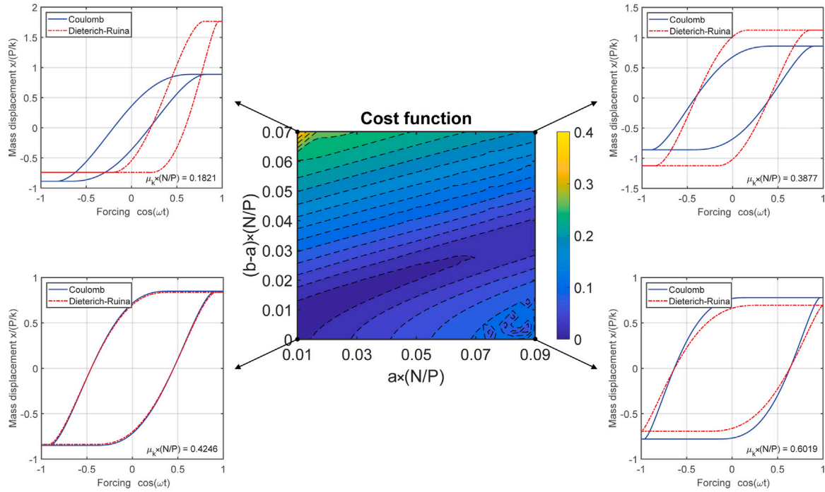
Fig. 15. Cost function obtained for optimal values of \bar{\mu}_k of the Amontons–Coulomb friction ( \bar{\mu}_s = \bar{\mu}_k ) model for r = 0.3 and \bar{\mu}_s = 0.4 (two-stop stick–slip motion with Dieterich–Ruina law). Comparison of the dynamic forcing–dynamic displacement graph obtained with the Amontons–Coulomb law’s ( \bar{\mu}_s = \bar{\mu}_k ) and Dieterich–Ruina law at the 4 corners of the parameter space.
