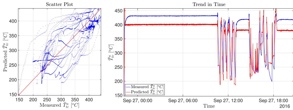
Figure 10. Scatter plot (measured vs predicted) and trend in time for \bar{T}_{tc}^a using a PM with \Delta = 0 . (This figure is available in colour online.)
