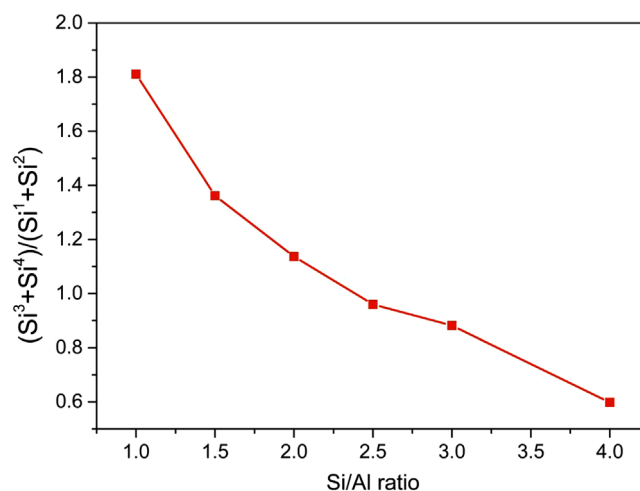
FIGURE 11 (Si^3 \text{ and } Si^4)/(Si^1 \text{ and } Si^2) as a function of Si/Al ratio
