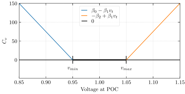
Fig. 2. Example plot of the Voltage penalty C_v , with parameters \beta_0 = 1425 , \beta_1 = 1500 , \beta_2 = 1575 , v_{min} = 0.95 and v_{max} = 1.05 . Values of voltage magnitudes outside technical limits at POC results in additional costs for the agent.
