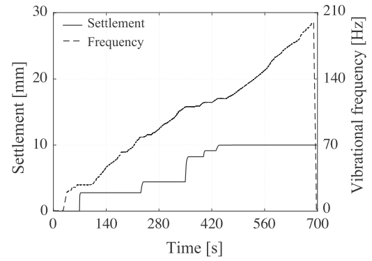
(b) Excitation frequency and displacements, Test 72.
