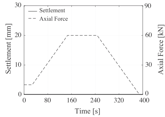
(b) Slip-joint capacity static test, Test 9.
