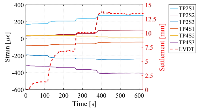
(b) Installation test 1 on cone-set 1, TP.
