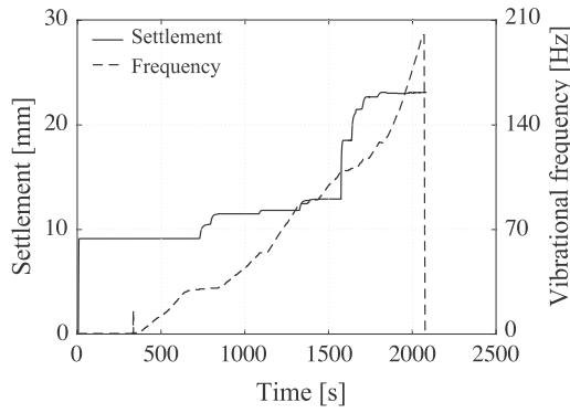
(a) Excitation frequency and displacements, Test 12.
