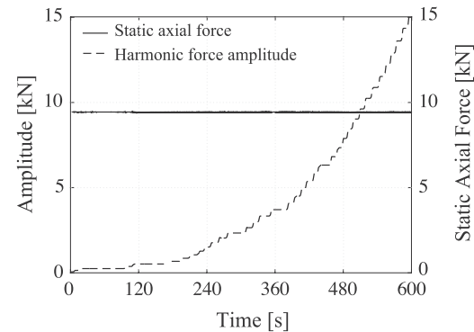
(b) The applied dynamic and static force, Test 1.
