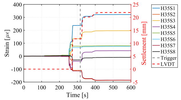
(b) Installation test 16 on cone-set 2, TP.
