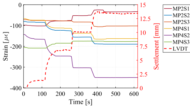
(a) Installation test 1 on cone-set 1, MP.
