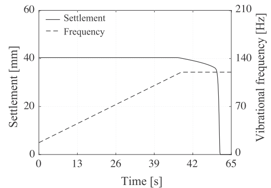
(b) Constant increase, Test 76.
