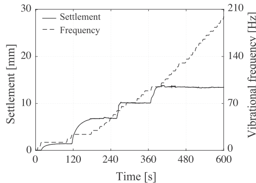
(a) The settlement of the upper cone and the vibrational frequency, Test 1.
