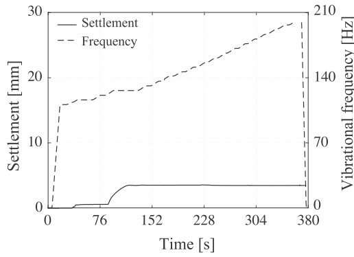
(a) Slow step wise frequency increase, Test 8.
