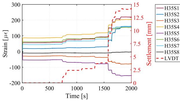
(a) Installation test 12 on cone-set 2, TP.
