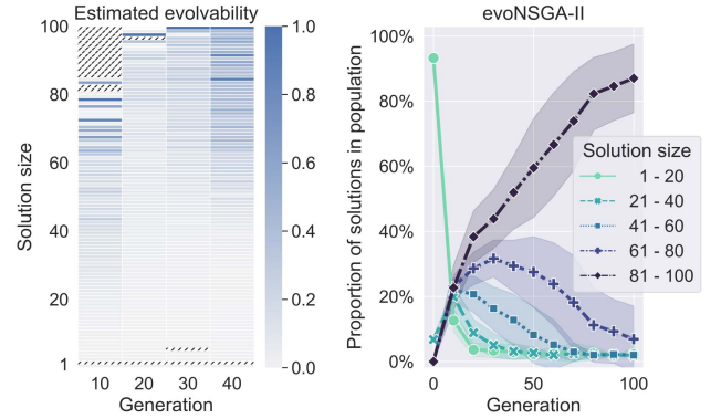
Figure 4: Left: Each column of the heat-map shows, for a given generation, the average evolvability between crossover and mutation computed with the workflow of Sec. 3.2 on Airfoil, and normalized across solution size (dashed entries represent absent sizes). Right: Proportions of solutions of different sizes in evoNSGA-II during 30 evolutions on Airfoil (lines are means, shaded areas are standard deviations).
