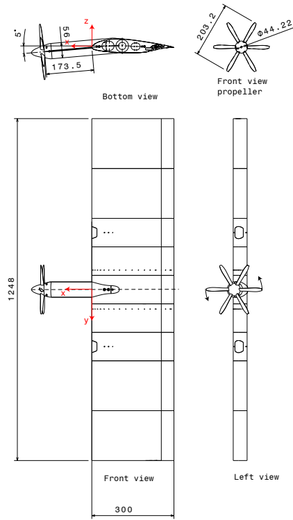
Fig. 4 Technical drawing of wing model. Dimensions in mm .
