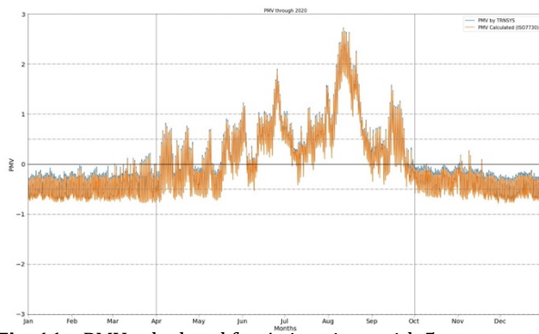
Fig. 11 – PMV calculated for 4 situations with 5 calculators
