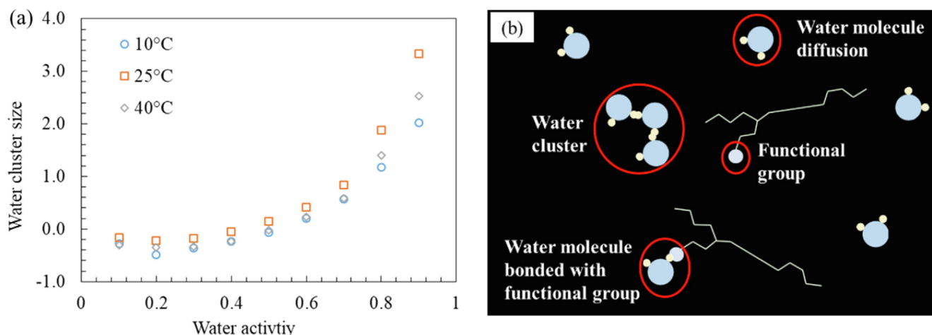
Fig. 17. (a) Evolution of mean water cluster size with water activity for the B1 binder determined by the Zimm-Lundberg model. (b) water transport and clustering mechanisms in bitumen.
