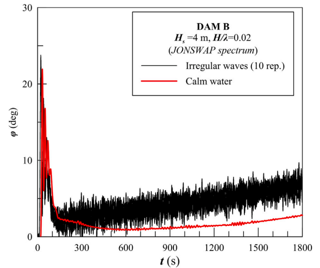
Fig. 14. Roll angle time-trace for DAM B in calm water and with H_s of 4 m. (For interpretation of the references to colour in this figure legend, the reader is referred to the web version of this article.)
