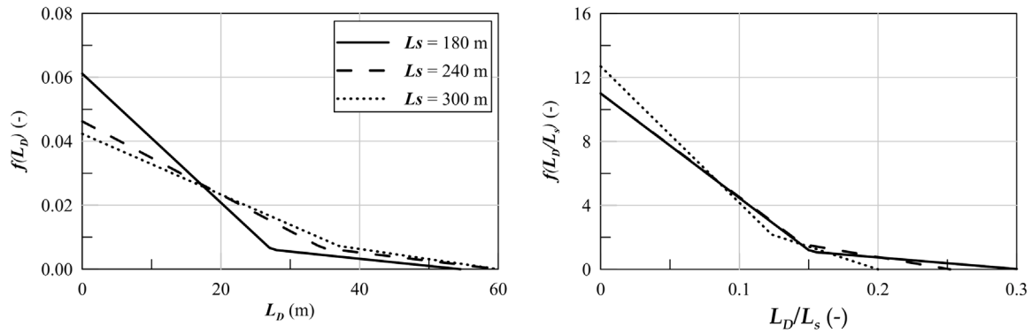
Fig. 1. Probability density functions of the dimensional (left) and non-dimensional (right) length of potential damage for a C00 collision.
