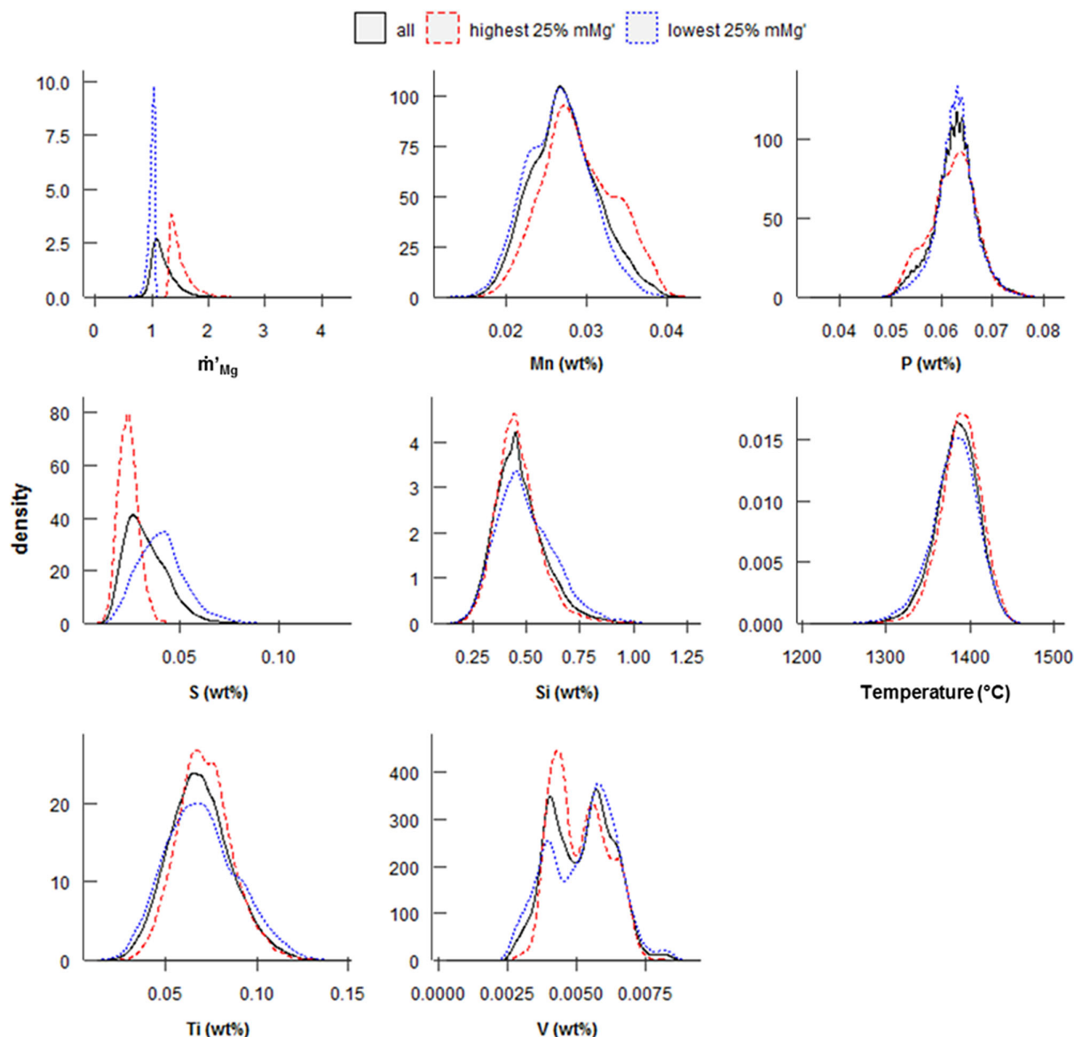
Figure 2. Distribution of the plant data from Tata Steel, IJmuiden, for the key parameters. Black solid lines show all data, the red dashed lines include only the data with the highest 25% m'_{Mg} and the blue dotted lines include only the data with the lowest 25% m'_{Mg} .
