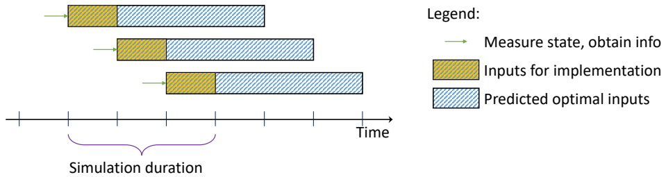
FIGURE 2.3: An MPC controller regularly gathers information and recomputes the optimal sequence of inputs for the prediction horizon. Only the first part of the plan is implemented.
