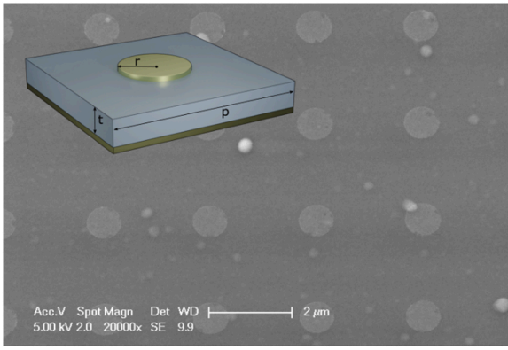
Fig. 8. (a) Structure of the unit cell of the metamaterial design with a circular metal patch with radius r = 450 - 550\text{nm} , unit cell side-length P = 3\mu\text{m} and \text{SiO}_2 dielectric thickness t = 170\text{nm} . (b) SEM of the realized r = 450\text{nm} metasurface.
