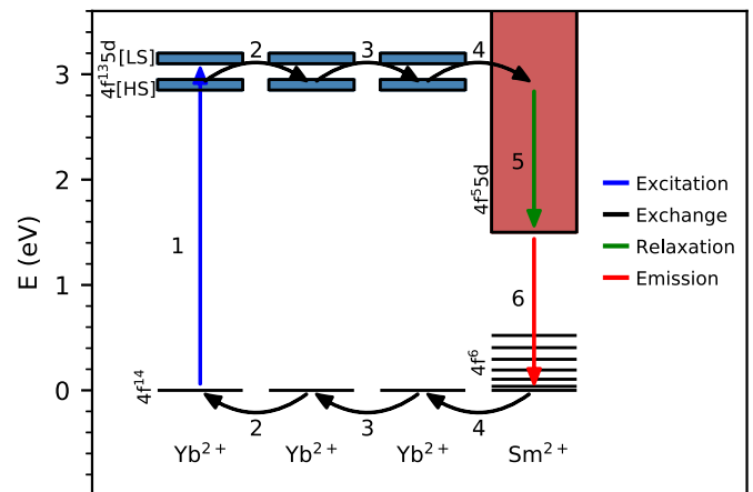
Fig. 1. Schematic of the energy transfer processes from \text{Yb}^{2+} to \text{Sm}^{2+} . After initial excitation of an \text{Yb}^{2+} ion, the excitation energy migrates over neighbouring \text{Yb}^{2+} ions until it is transferred to \text{Sm}^{2+} from which emission is observed. The energy scale on the y-axis corresponds to approximate values for the samples studied in this work.
