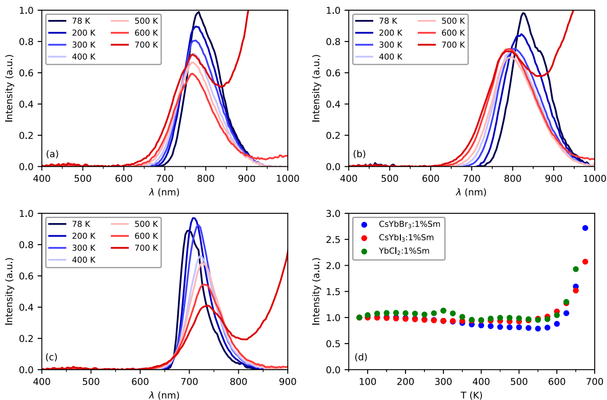
Fig. 2. X-ray excited emission spectra of (a) \text{CsYbBr}_3:1\%\text{Sm} , (b) \text{CsYbI}_3:1\%\text{Sm} and (c) \text{YbCl}_2:1\%\text{Sm} . (d) Shows the emission intensity of all samples integrated from 600 nm to 1000 nm against temperature.
