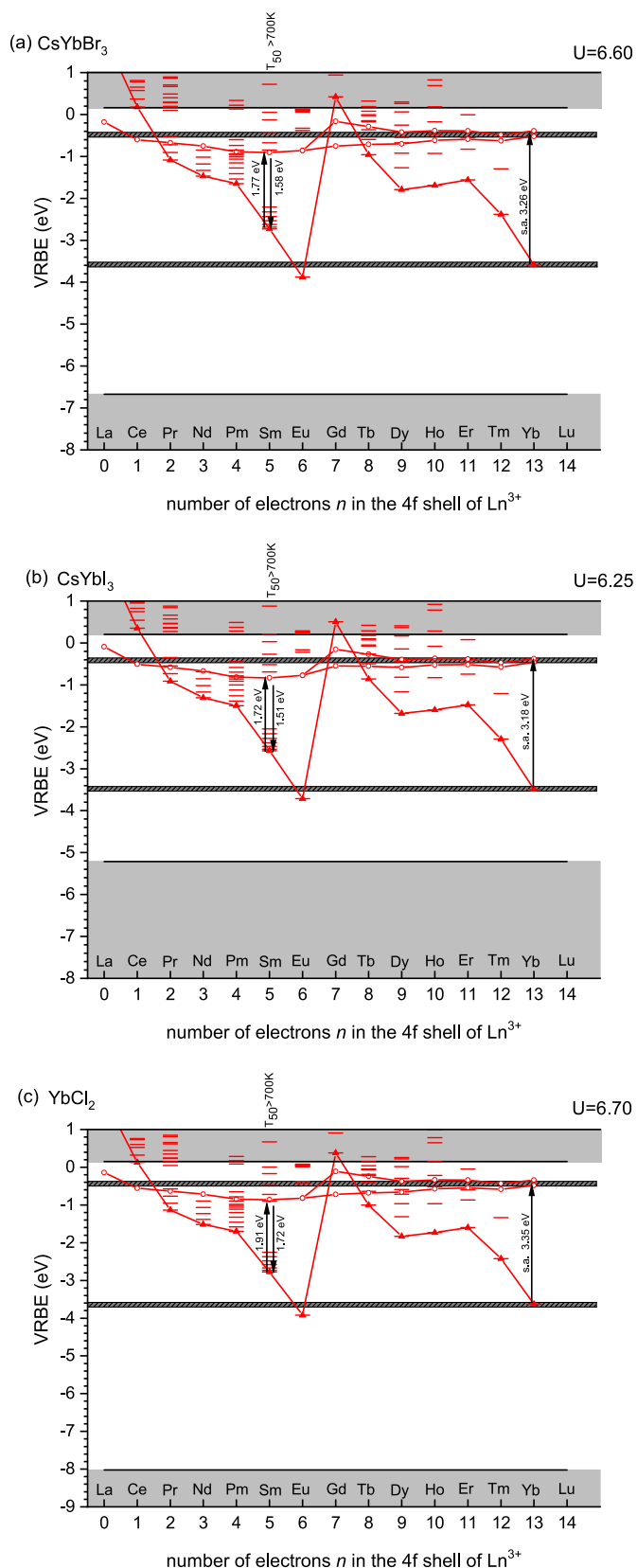
Fig. 7. VRBE diagrams of (a) CsYbBr 3 , (b) CsYbI 3 and (c) YbCl 2 . The dark grey horizontal lines indicate the 4f 14 ground state and 4f 13 [ 2 F 7/2 ]5d 1 excited states and are drawn to indicate that Yb 2+ is part of the host compound.
