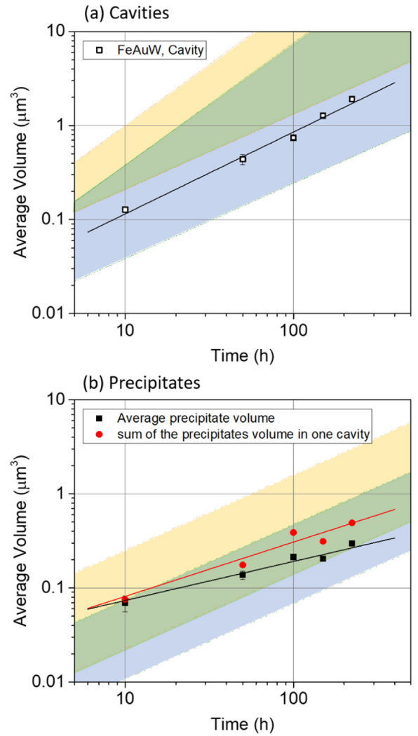
Fig. 11. Average volume \langle V \rangle of (a) the cavities and (b) the precipitates as a function of time. The lines are fits to \langle V \rangle = k t^n . The blue and yellow shaded areas show the range of Fe-W and Fe-Au alloys, respectively and the green areas for the overlap. The upper and lower limits represent the linked and isolated features, respectively. In (b), the black data points are the average volumes of all the precipitates, while the red ones show the average value for the summed volume of the precipitates in each cavity. The fitting parameters are listed in Table S2 (supplementary information) (For interpretation of the references to color in this figure legend, the reader is referred to the web version of this article.).
