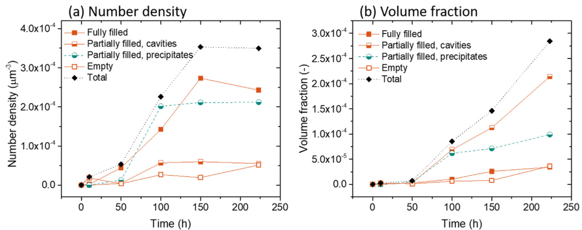
Fig. 8. Time evolution of (a) the number density and (b) the volume fraction of the cavities. Three groups of cavities (empty, partially-filled and fully-filled) are categorised based on their degree of filling. The data for the precipitates in the partially filled cavities are also presented for comparison.
