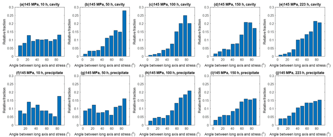
Fig. 9. Distribution of the angle between the long axis of the cavities ((a–e)) / precipitates ((f–j)) and the loading direction for different creep times. An angle of 90° indicates that the corresponding cavity / precipitate is oriented perpendicular to the load direction.
