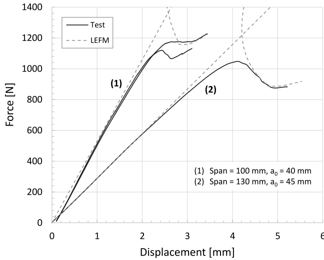
Fig. 16. ENF experimental results versus analytical solution.
