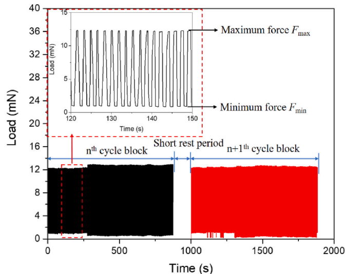
Fig. 7. Illustration of cyclic load history applied in MCB fatigue tests.
