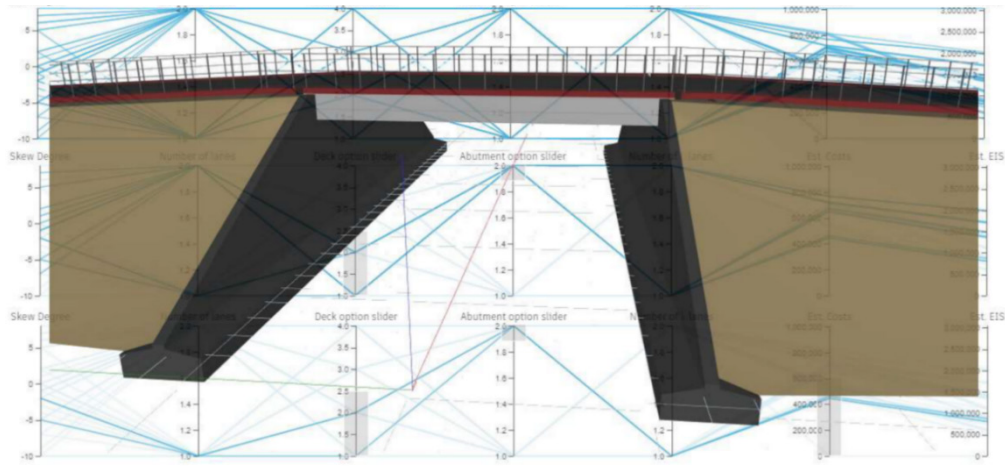
FIG 2. A PROTOTYPE GENERATIVE DESIGN SYSTEM FOR AUTOMATED CONCRETE VIADUCTS DESIGNING (SKAKUN 2021)
