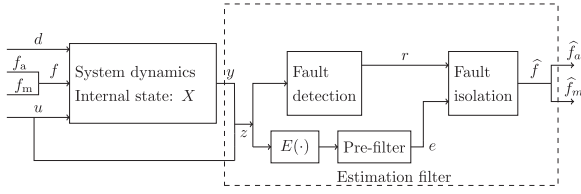
Fig. 1. Block diagram of the proposed estimation filter.
