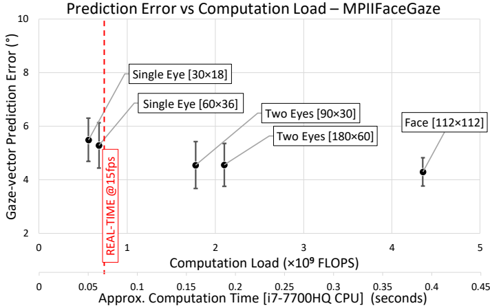
(a) MPIIFaceGaze
