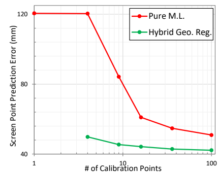
(a) MPIIFaceGaze
