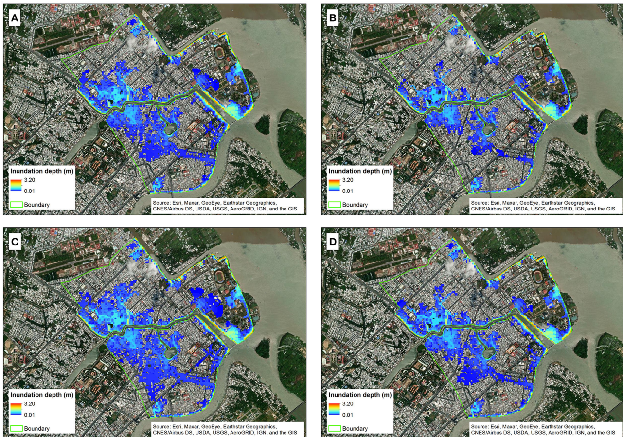
FIGURE 10 | Flood hazard maps (i.e., maximum flood depths) for the 100-year return period of water level for hydrograph shape Pattern 1 (left) and Pattern 2 (right) under RCP 4.5 ( A,B ) and RCP 8.5 ( C,D ) (without land subsidence). The inundated area (for cells with maximum inundation depths \geq 0.02 m) for RCP 4.5 and RCP 8.5 corresponding to Pattern 1 are 1.96 and 2.30 km 2 , respectively, while for Pattern 2 are 1.41 and 1.81 km 2 , respectively.
