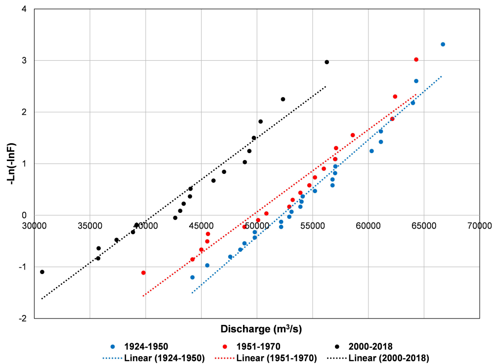
FIGURE 16 | Gumbel distribution of discharge peaks at Kratie corresponding to three periods (1924–1950), (1951–1970), and (2000–2018).
