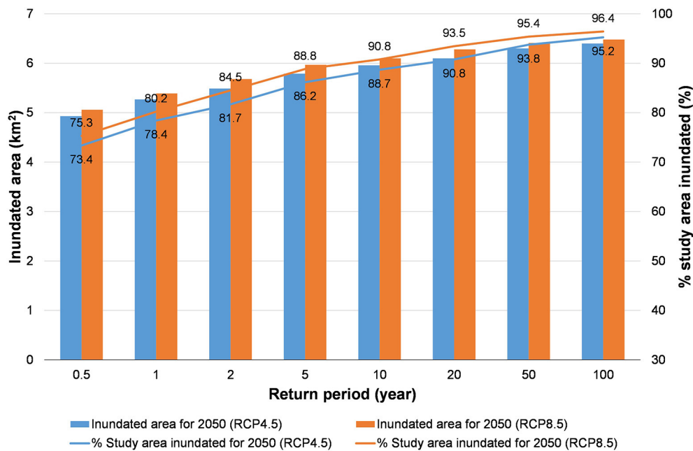
FIGURE 14 | The inundated area and percentage of the flooded area relative to total study area (also indicated by numerics along the solid lines in this figure) corresponding to each return period of water level for model scenarios (including land subsidence).
