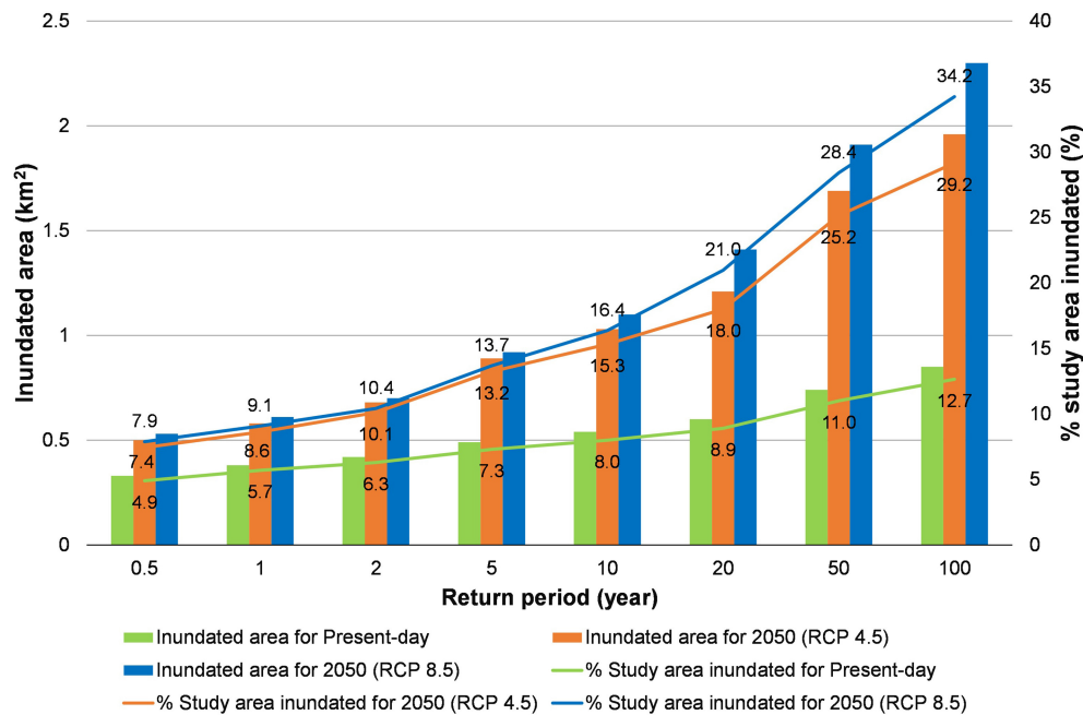
FIGURE 12 | The inundated area and percentage of the flooded area relative to total study area (also indicated by numerics along the solid lines in this figure) corresponding to each return period of water level (without land subsidence).
