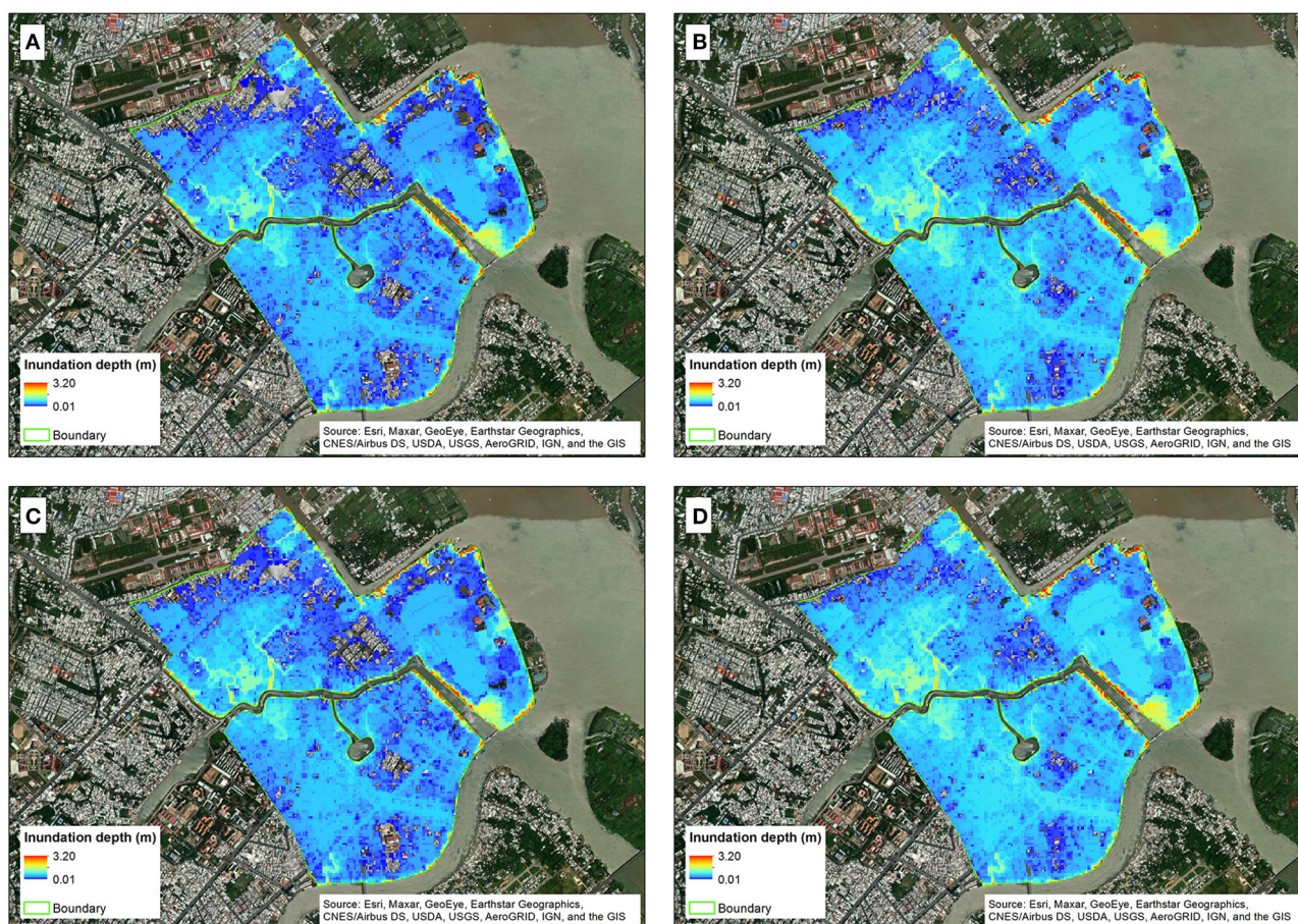
FIGURE 13 | Flood hazard maps corresponding to 5 year and 100 return period of water level for 2050 under RCP 4.5 (model scenario #2) (A,B), and RCP 8.5 (model scenarios #4) (C,D), respectively.
