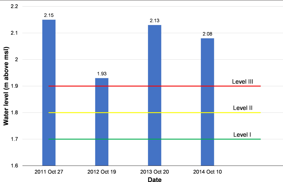
FIGURE 2 | Highest measured water levels of the flooding years since 2000 and flood water level alarms in Can Tho (flood water level alarms are implemented following Decision No. 632/QĐ-TTg issued on May 10th, 2010).
