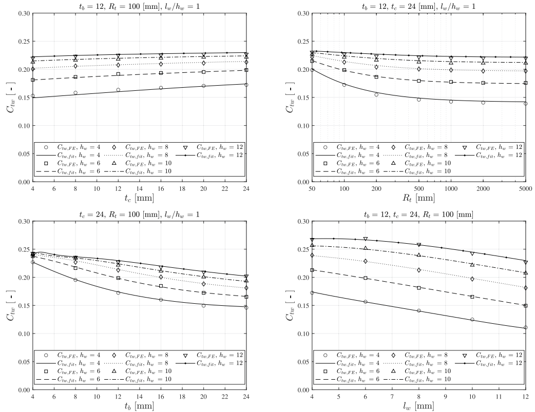
Fig. 10. Required C_{lw} value and fit estimate for a DS welded T-joint varying t_b , t_c , l_w , h_w and R_t .
