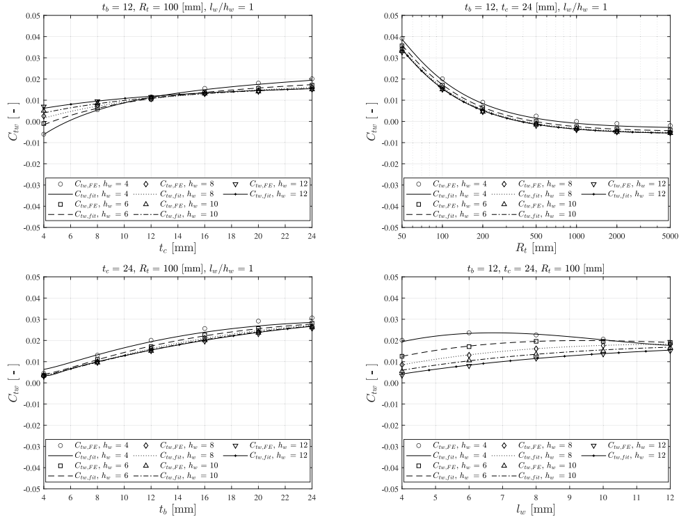
Fig. 17. Required C_{tw} value and fit estimate for a DS welded cruciform joint, varying t_b , t_c , l_w , h_w and R_t .
