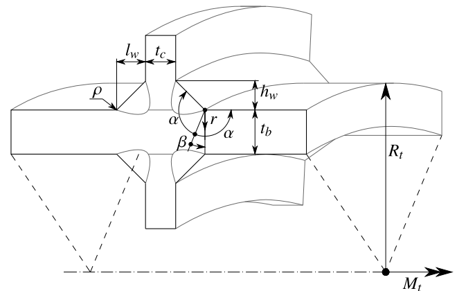
Fig. 15. DS welded cruciform joint showing symmetry with respect to (t_b/2) , either in a tubular or planar ( R_t \rightarrow \infty ) structure.
