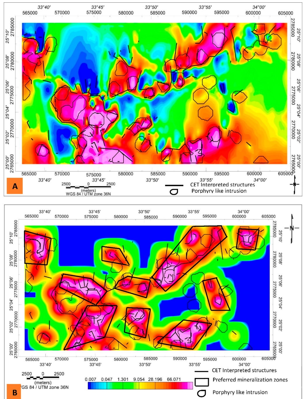
Figure 10. (A) The circular boundary porphyry tracing and skeleton of vector lineaments are superimposed on the RTP map of the study region. (B) Figure illustrating the OE map, vectorized lineaments (black lines), the circular boundary porphyry tracing (black circular), and prospective areas (in the black line) of the study area.
