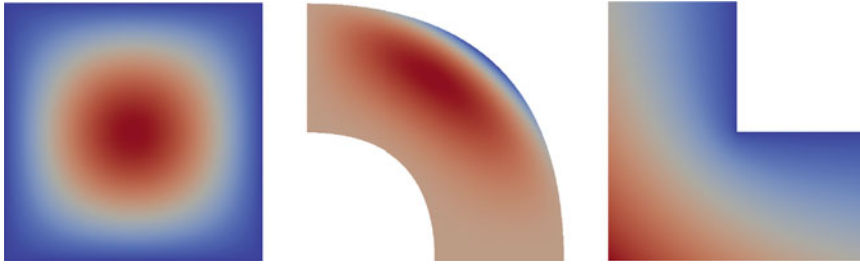
Fig. 5 Exact solutions on the three domains of the considered benchmarks
