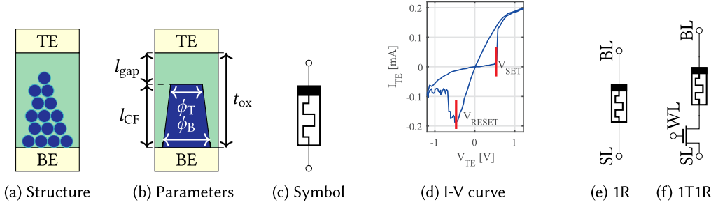
Fig. 1. RRAM device.
