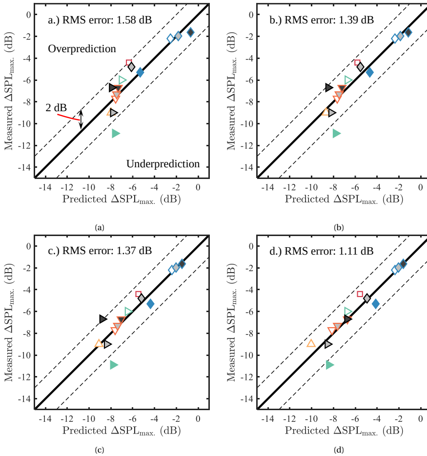
Figure 7.6: Prediction accuracy of the selected individuals in the Pareto front of the symbolic regression modeling trial 1.
