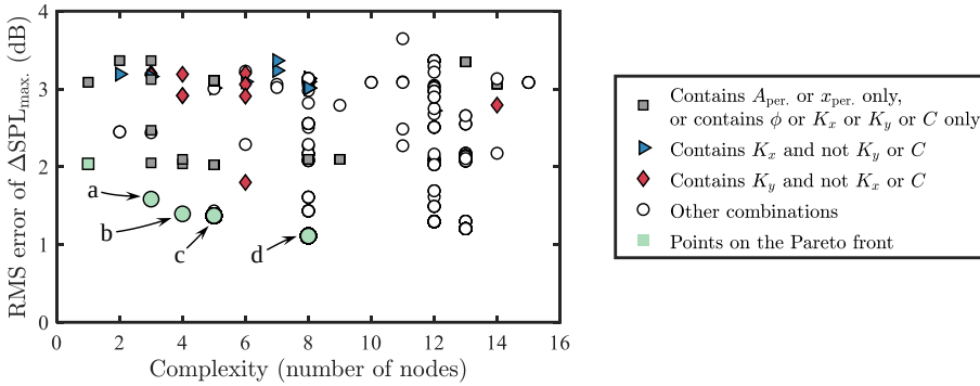
Figure 7.5: Functional complexity and prediction accuracy of the final-generation population of the symbolic regression modeling trial 1.
