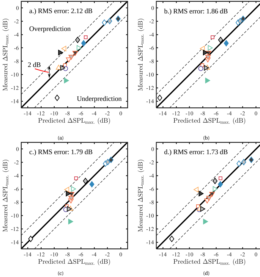
Figure 7.8: Prediction accuracy of the selected individuals in the Pareto front of the symbolic regression modeling trial 2.
