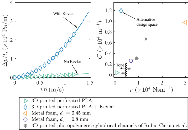
Figure 6.2: Left: measured static pressure drop \Delta p across the 3D-printed perforated PLA samples having the thickness t_s = 60 mm with and without the Kevlar sheet for 15 different Darcy velocities v_D , including the curve-fitting of Eq. (2.23) to the measured data. Right: measured r versus C for the permeable material samples tested and those from permeable materials in literature.
