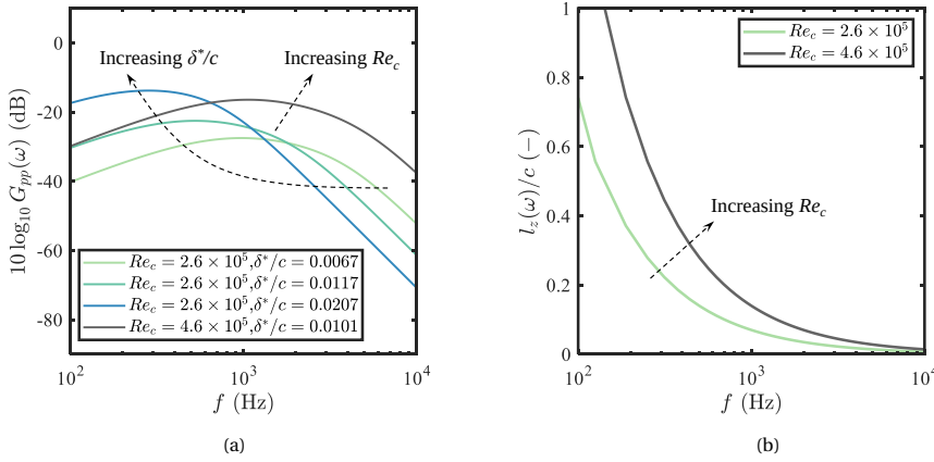
Figure 2.3: (a) Example of the predicted G_{pp}(\omega) using the Kamruzzaman's model for a NACA 0018 airfoil at x/c = -0.02 for varying Re_c and \delta^* and (b) Example of the predicted l_z(\omega) using the Corcos' model for the same NACA airfoil.
