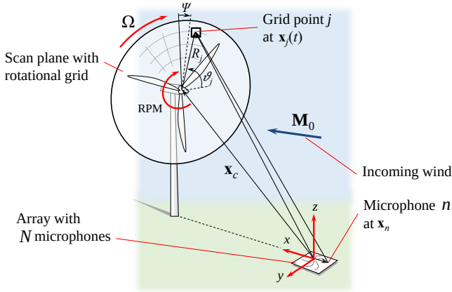
Figure 4.6: Schematic of a microphone-array noise measurement of a wind turbine and notations used in the ROSI beamforming.
