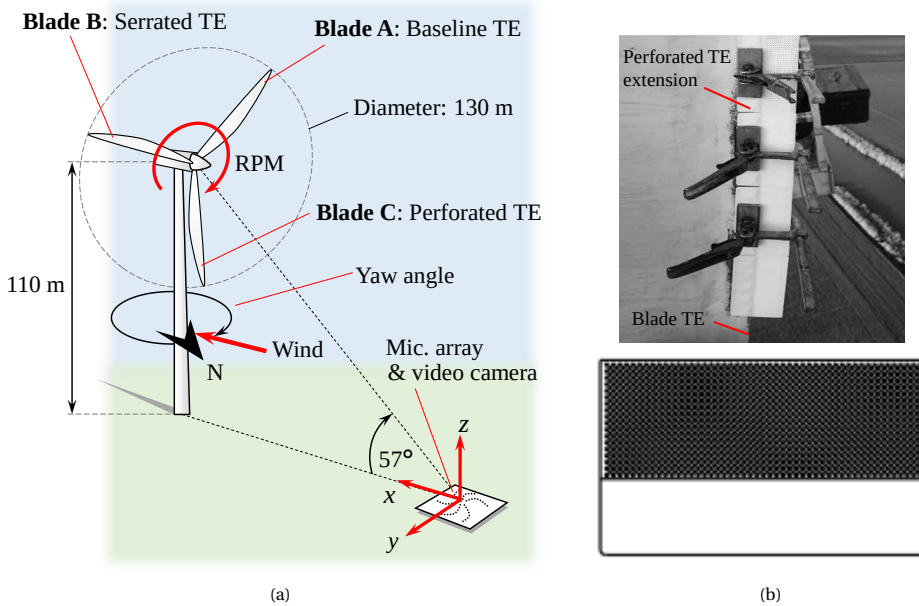
Figure 8.1: Noise measurement set up of a wind turbine with the three different blade TE configurations: (a) Schematic (not to scale) and (b) photograph and drawing of the perforated TE extension.
