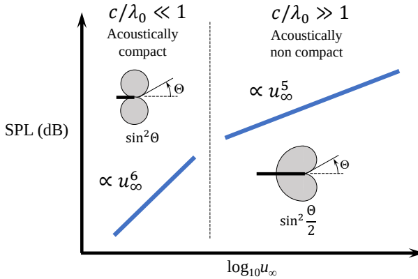
Figure 2.1: Theoretical noise emission of a turbulent flow with a solid body present.
