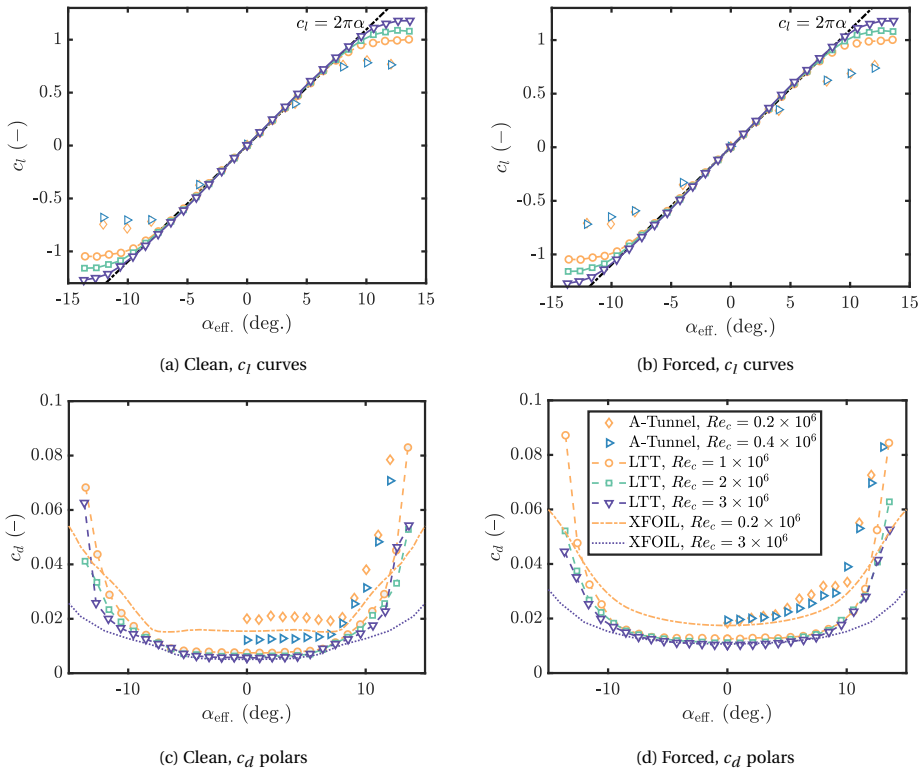
Figure 5.7: Comparison of c_l curves and c_d polars from the A-Tunnel and the LTT tests of the baseline NACA 63 3 -018 airfoil at various Re_c .
