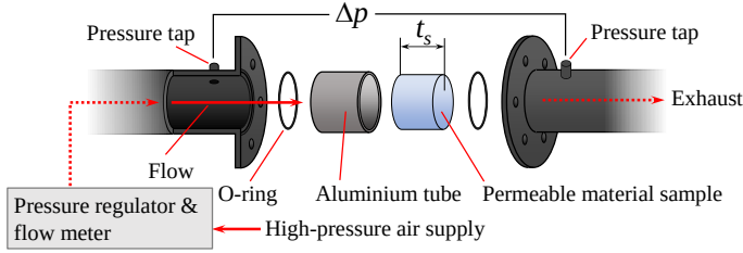
Figure 2.4: Schematic of the permeability test set up.
