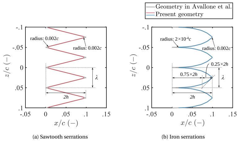
Figure 5.1: Drawings of the TE serrations used on the airfoil compared to the geometry used in the simulation of Avallone et al. [141].
