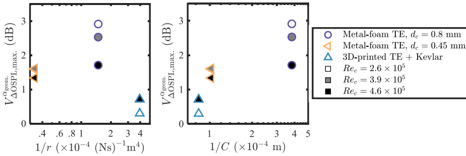
Figure 6.9: Noise attenuation variability with the geometrical angle of attack of the airfoil with various permeable TE inserts at various chord-based Reynolds numbers as functions of the flow resistivity (left) and form drag coefficient (right).
