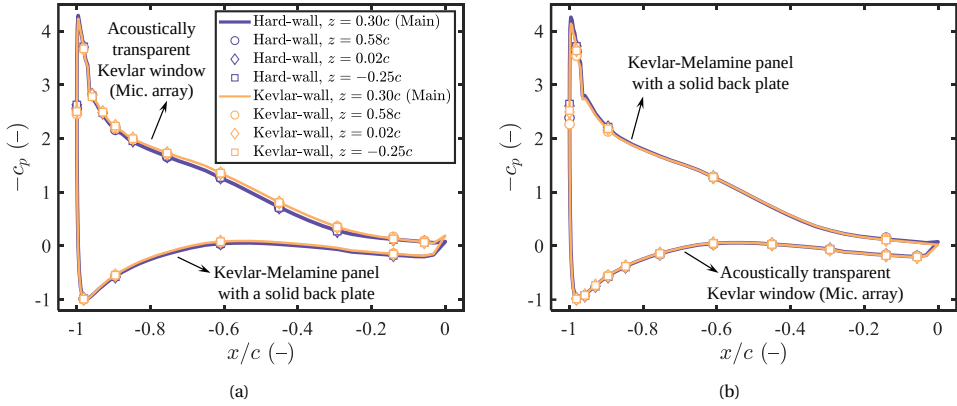
Figure 3.8: Comparison of c_p distribution obtained from multiple spanwise pressure tap rows on the baseline NACA 633-018 airfoil in the LTT test section with hard-wall and Kevlar-wall configurations at Re_c = 3 \times 10^6 for (a) \alpha_{\text{eff}} \approx 10^\circ and (b) \alpha_{\text{eff}} \approx -10^\circ .
