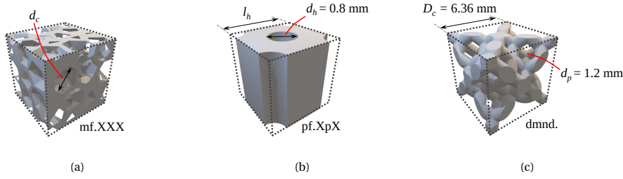
Figure 7.2: Schematic of the permeable materials: (a) Porous metal foam, (b) Perforated channels, and (c) Diamond-lattice structure.
