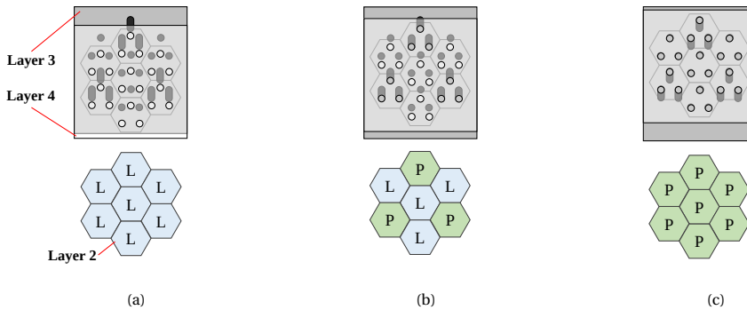
Figure C.2: Operational modes of the hybrid permeable liner (L = liner and P = permeable structure).
