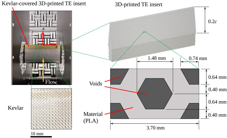
Figure 6.1: 3D-printed permeable TE insert covered by a Kevlar fabric, installed on a NACA 0018 airfoil model with a close-up view on the Kevlar fabric, the 3D-printed TE insert, and the perforated pattern.
