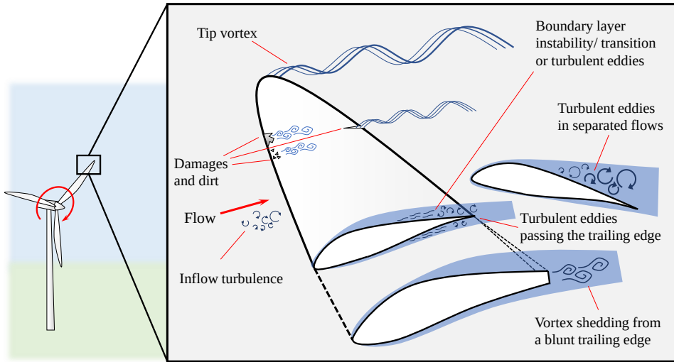
Figure 1.6: Schematic of possible flow-blade interaction mechanisms that contribute to aerodynamic noise emissions from a wind turbine (Adapted from Wagner et al. [26] and Blake [27]).
