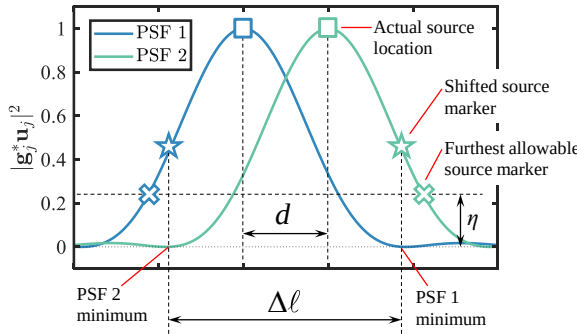
Figure 4.4: Schematic of two closely-spaced sound sources resolved by HR-CLEAN-SC after the source markers have been shifted. The source marker constraint \eta is also shown.
