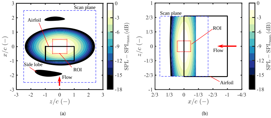
Figure 4.3: PSFs of a simulated point source placed at the origin (airfoil trailing edge center) for a 1/3-octave frequency band centered at 1 kHz for the (a) A-Tunnel set up and (b) LTT set up.
