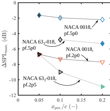
Figure 7.3: \Delta\text{SPL}_{\text{max}} versus x_{\text{per.}}/c for various airfoil geometries.
