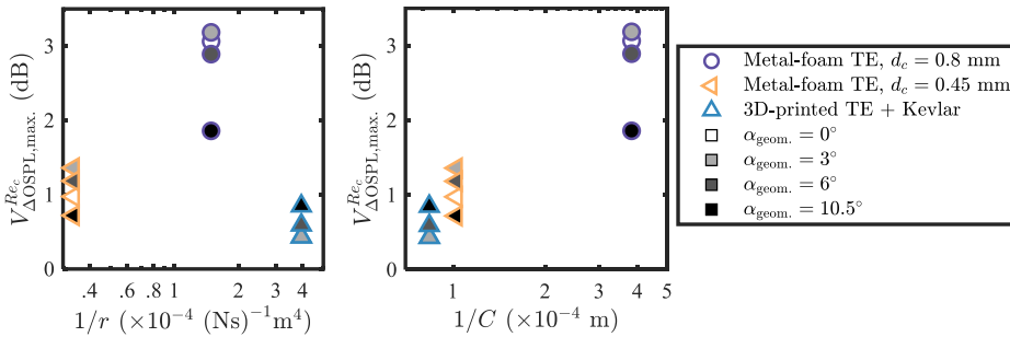
Figure 6.10: Noise attenuation variability with the chord-based Reynolds number of the airfoil with various permeable TE inserts at various geometrical angles of attack as functions of the flow resistivity (left) and form drag coefficient (right).
