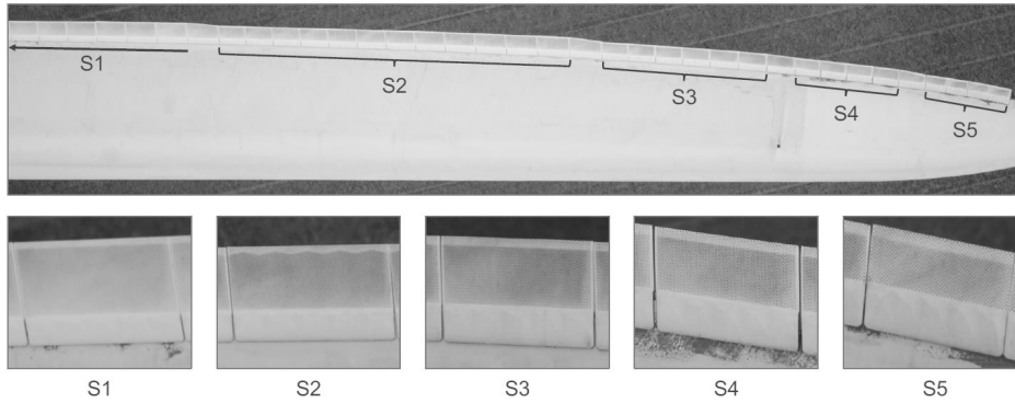
Figure 8.4: Drone photographs of the perforated TE extensions approximately one month after installation.
