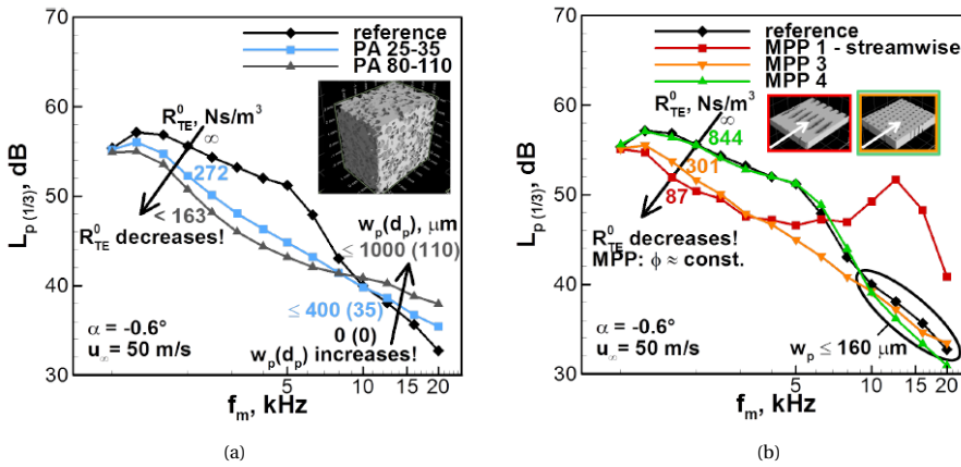
Figure 2.5: Far-field noise spectra of a DLR F16 airfoil with baseline and permeable trailing edges for different permeable material groups: (a) Porous Aluminum (PA) and (b) Micro Perforated Plates (MPP), reproduced from Herr et al. [109] with permission from the corresponding author. The notations used in this figures mean the following: R_{TE}^0 : flow resistivity, w_p : pore width, d_p : effective pore size, \phi : porosity, \alpha : angle of attack, u_\infty free-stream flow speed, L_{p(1/3)} : far-field noise level in 1/3-octave band, and f_m : middle frequency.
