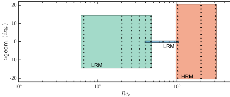
Figure 5.3: Illustration of the conditions tested in the test campaigns. The circle and square marks represent the conditions measured during the campaigns with LRM using the 3.5c \times 2c nozzle and the 1.25c \times 2c nozzle in the A-Tunnel, respectively. The triangular marks represent the experiments carried out with the HRM in the LTT.
