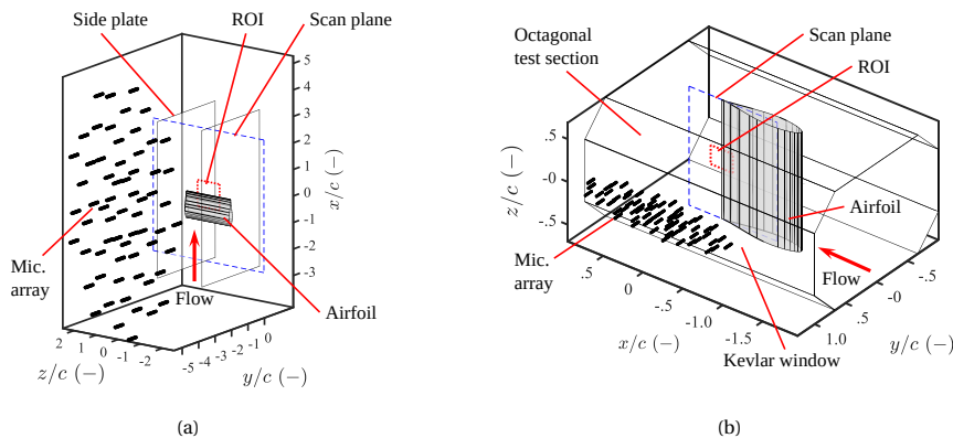
Figure 4.1: Microphone arrays for noise measurements of an airfoil in wind tunnels (a) A-Tunnel and (b) LTT.
