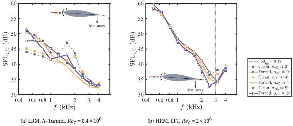
Figure 5.11: SPL spectra for the airfoils with baseline TE considering natural and forced transition configurations at various \alpha_{eff} .
