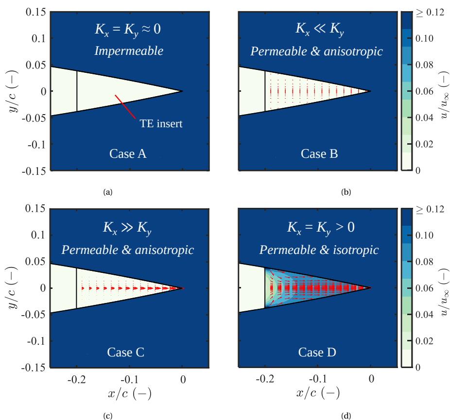
Figure D.1: Close-up view of the velocity field within a permeable TE insert having different permeabilities on a NACA 0018 airfoil predicted by the MSEM for zero-degree angle of attack.
