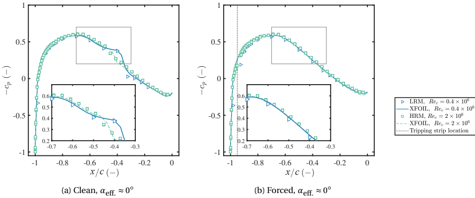
Figure 5.4: Comparison of c_p distributions from the A-Tunnel and the LTT tests of the baseline NACA 633-018 airfoil with XFOIL predictions at various Re_c and \alpha_{\text{eff.}} \approx 0^\circ .
