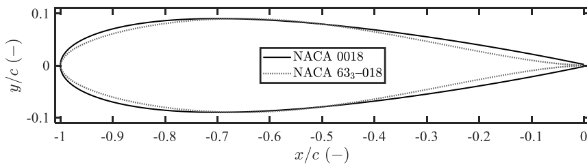
Figure 3.1: Airfoil profiles considered.
