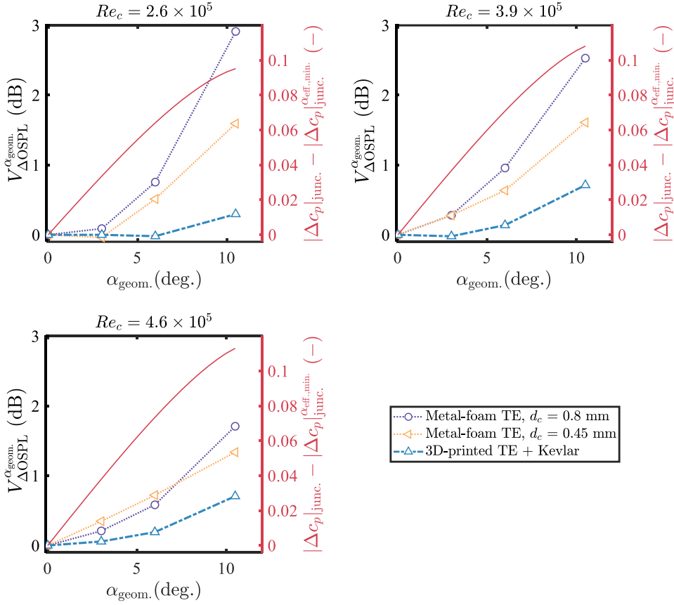
Figure 6.6: Noise reduction variability with respect to the angle of attack of various permeable TE inserts at different chord-based Reynolds numbers relative to the noise reduction at zero-degree geometrical angle of attack.
