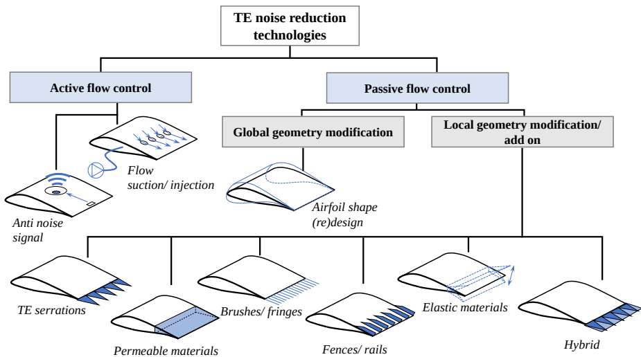
Figure 1.7: Trailing-edge noise reduction approaches.
