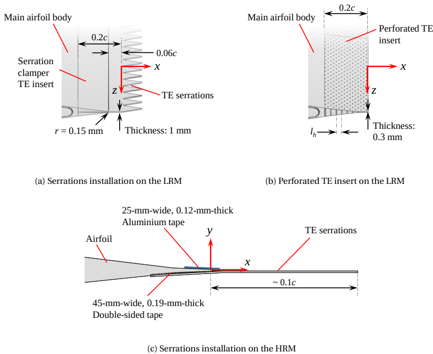
Figure 5.2: TE add-on installations on the airfoils.
