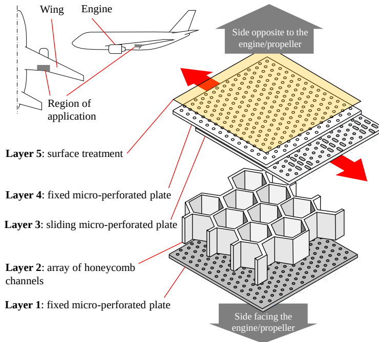
Figure C.1: Schematic of the hybrid permeable liner design concept.
