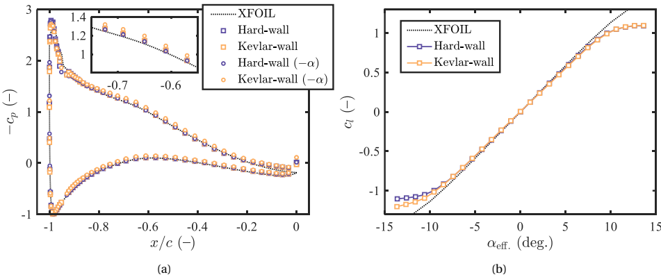
Figure 3.7: Aerodynamic coefficients of the 0.9-m-chord NACA 633-018 airfoil in the LTT test section with hard-wall and Kevlar-wall configurations at Re_c = 3 \times 10^6 compared to XFOIL predictions: (a) c_p for \alpha_{\text{eff.}} \approx \pm 8^\circ and (b) c_l polar.
