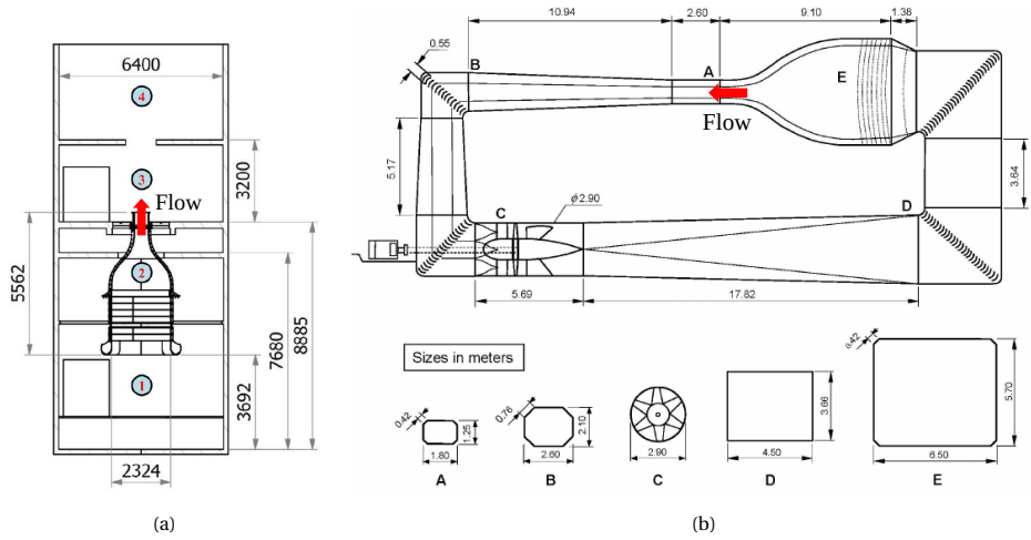
Figure 3.3: Schematics of the wind tunnels. The arrow specifies the flow direction towards the location where the airfoil model is installed: (a) A-Tunnel, the numbers label ① the settling chamber, ② the 3D-printed contraction, ③ the anechoic chamber, and ④ the fan and collector room (Scales in mm), reproduced from Merino-Martínez et al. [151] with permission from the corresponding author; (b) LTT (Scales in m), reproduced from Timmer [147] with permission from the author.
