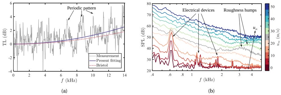
Figure B.2: (a) Transmission losses (TL) through the Kevlar sheet and (b) Background noise SPL spectra measured in the LTT versus flow speeds u_\infty .
