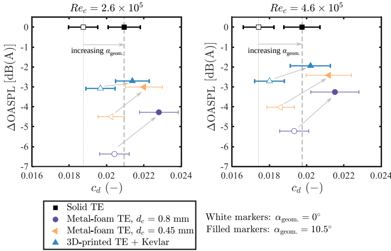
Figure 6.16: Comparison of noise attenuation and drag coefficients provided by all the permeable TE inserts at different combinations of the chord based Reynolds numbers and geometrical angles of attack.
