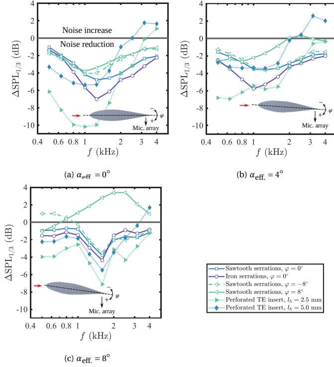
Figure 5.15: One-third octave band sound pressure level noise reduction spectra for the LRM under forced transition condition with TE add-ons at Re_c = 0.4 \times 10^6 and various \alpha_{eff} .
