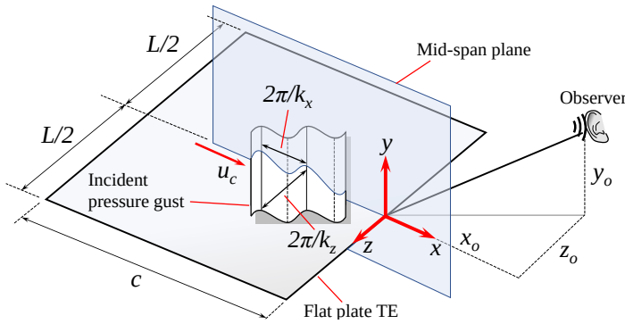
Figure 2.2: Schematic of an incident pressure gust approaching a straight TE of a flat plate.
