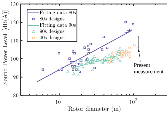
Figure 1.3: Sound power levels of wind turbines with different rotor diameters classified by the year they were designed. The 'Present measurement' refers to the measurement presented in Section 1.3.
