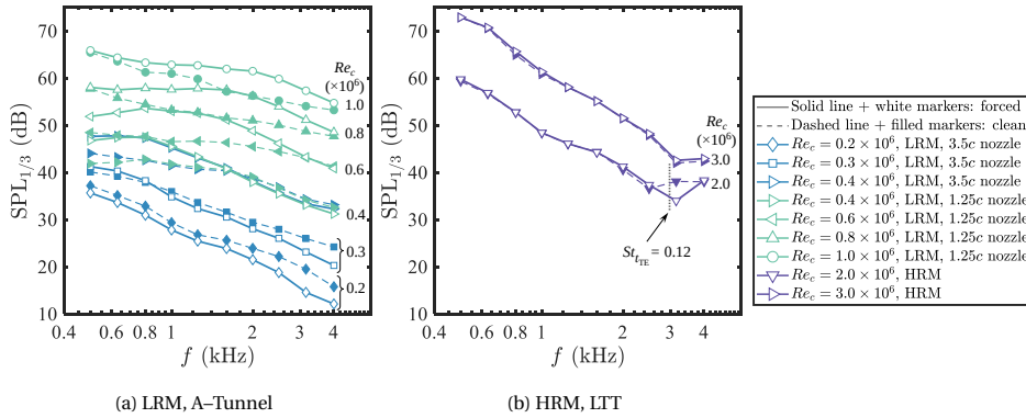
Figure 5.10: SPL spectra for the airfoils with baseline TE at various Re_c and \alpha_{eff} \approx 0^\circ considering natural and forced transition configurations.
