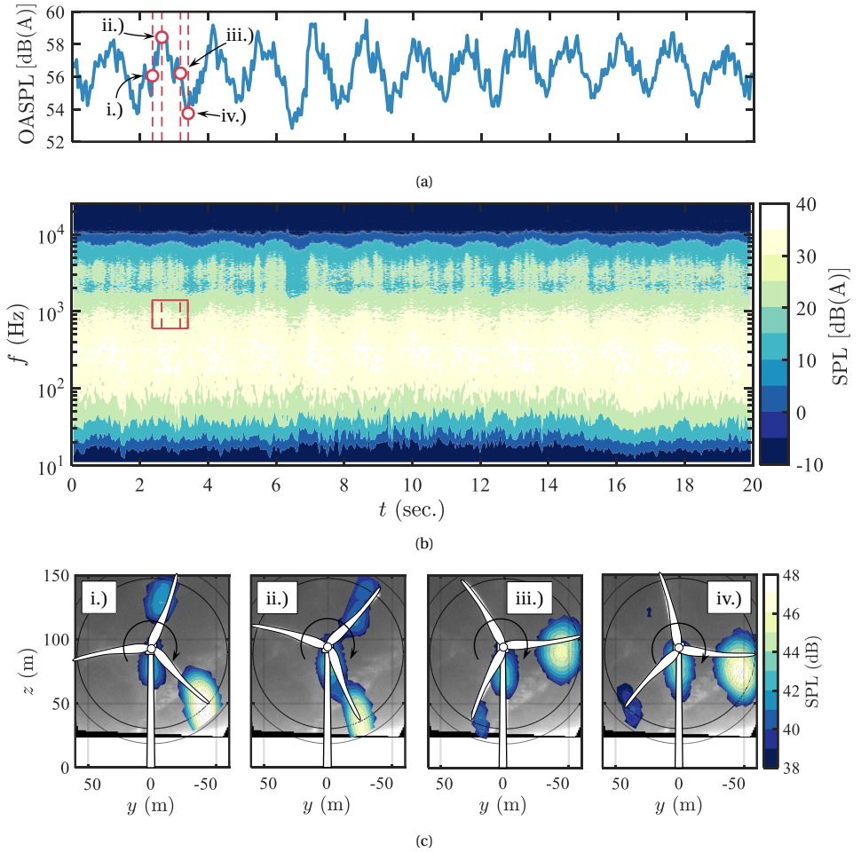
Figure 1.5: Wind turbine noise in a 20-second excerpt: (a) Time-series OASPL (b) spectrogram, and (c) instantaneous ROSI beamforming images at time instances and frequency range marked in (a) and (b).
