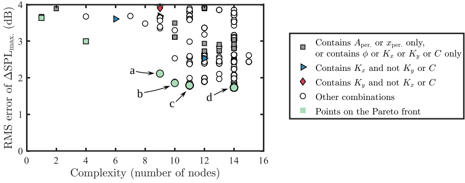
Figure 7.7: Functional complexity and prediction accuracy of the final-generation population of the symbolic regression modeling trial 2.
