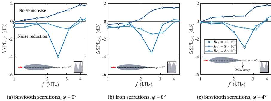
Figure 5.14: One-third octave band SPL noise reduction spectra for the HRM under forced transition condition with TE add-ons at various Re_c and \alpha_{eff} \approx 0^\circ .
