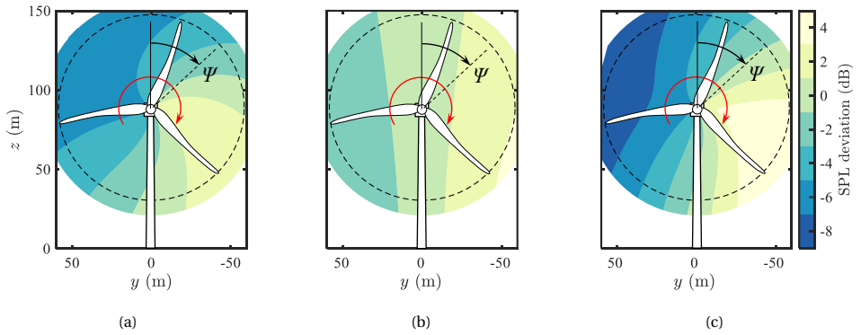
Figure 4.8: SPL deviation of the noise perceived from a wind turbine due to (a) the directionality (b) the convective amplification (c) the directionality and the convective amplification combined.
