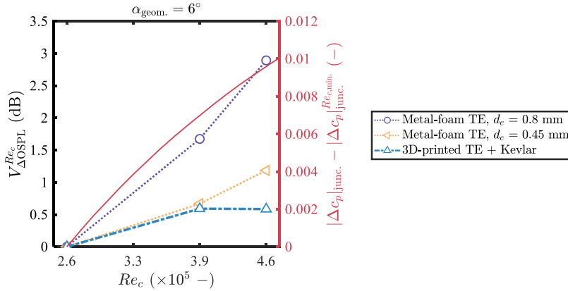
Figure 6.7: Noise reduction variability with respect to the chord-based Reynolds number of various permeable TE inserts at a geometrical angle of attack of 6 degree relative to the noise reduction at the lowest chord based Reynolds number.
