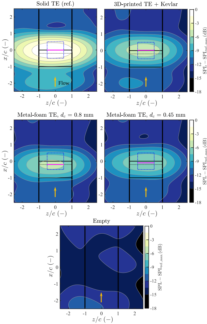
Figure 6.11: Source maps showing the relative SPL at Re_c = 2.6 \times 10^5 ( St_{\delta_s^* TE, ref.} \approx 0.12 ) and \alpha_{geom.} = 0^\circ for various permeable TE inserts. The levels are relative to the maximum SPL of the ‘reference’ solid TE case ( SPL_{ref, max.} ), i.e. \Delta SPL = SPL - SPL_{ref, max.} dB. The colorbars are identical and apply to all of the maps.
