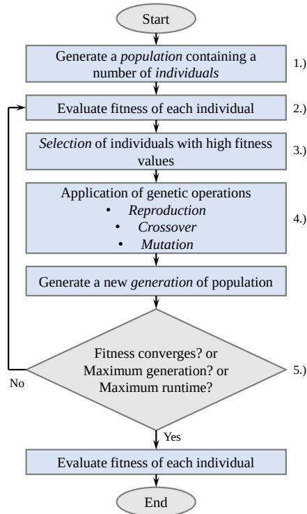
Figure 7.4: Flow diagram of the genetic programming.
