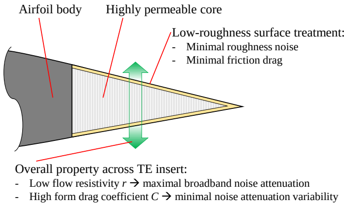
Figure 6.17: Proposed TE insert design concept for TBL-TE noise attenuation based on findings in the present study.
