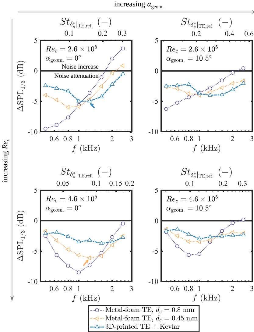
Figure 6.5: 1/3-octave band SPL spectra of various permeable TE inserts at different combinations of chord-based Reynolds numbers and geometrical angles of attack relative to those of the reference solid TE case ( \Delta\text{SPL}_{1/3} = \text{SPL}_{1/3} - \text{SPL}_{1/3, \text{ref.}} dB).
