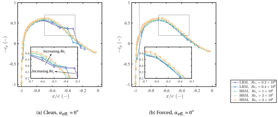
Figure 5.5: Comparison of c_p distributions from the A-Tunnel and the LTT tests of the baseline NACA 633-018 airfoil at various Re_c and \alpha_{\text{eff}} \approx 0^\circ .
