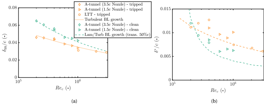
Figure 5.8: (a) \delta_{99}/c measured at X/c = -0.02 and \alpha_{\text{eff}} \approx 0^\circ compared against (corrected) scaling laws for turbulent and transitional boundary layers over a plate. The scaling laws are provided to guide the reader to the expected trend from the theory. (b) \delta^*/c measured at x/c = -0.02 and \alpha_{\text{eff}} \approx 0^\circ compared against predictions obtained with XFOIL.
