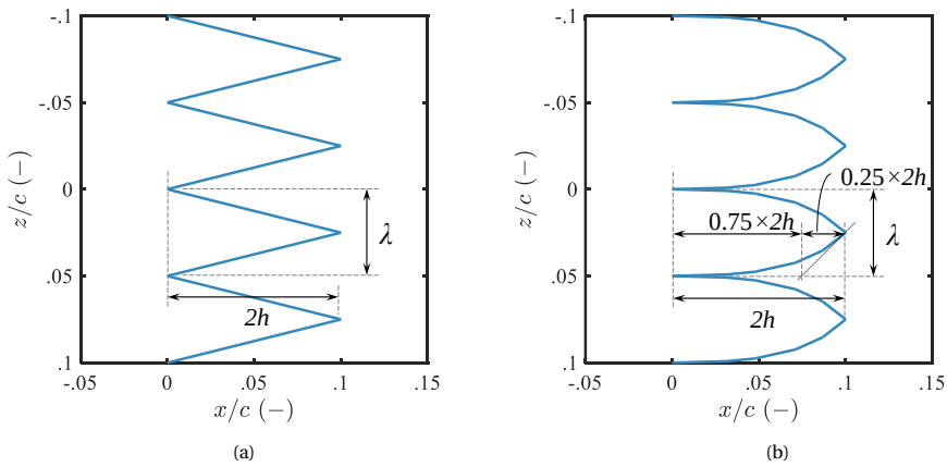
Figure 2.7: (a) Sawtooth serrations (b) Iron serrations.
