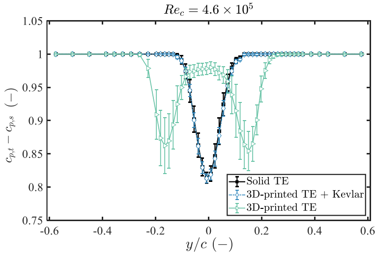
Figure 6.14: Wake profiles captured downstream of the airfoil with different TE inserts at Re_c = 4.6 \times 10^5 and \alpha_{\text{geom.}} = 0^\circ .
