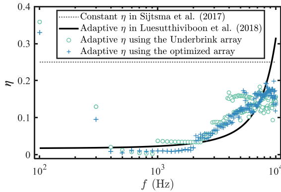
Figure 4.5: Value of \eta used in the Enhanced HR-CLEAN-SC algorithm versus frequency to resolve two closely-spaced sound sources from synthesized data using the Underbrink and optimized arrays, compared with \eta = 0.25 in the HR-CLEAN-SC algorithm [185] and the adaptive \eta based on the assumed MSL [175].
