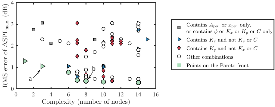
Figure 7.9: Functional complexity and prediction accuracy of the final-generation population of the symbolic regression modeling trial 3.
