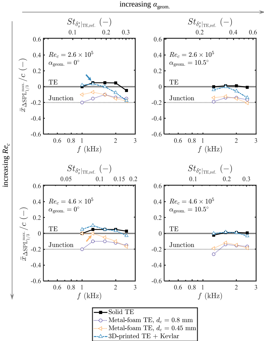
Figure 6.12: Streamwise locations of the maximum SPL from the source maps per frequency at different combinations of chord-based Reynolds numbers and geometrical angles of attack relative to the locations of the trailing edge (TE) and the junction between the solid and the permeable extents of the airfoil.
