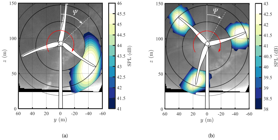
Figure 4.7: Source maps for a wind turbine obtained by (a) CTDBF ( \Omega = 0 rad/s) and (b) ROSI ( \Omega = 1.42 rad/s) beamforming calculated for a full rotation.
