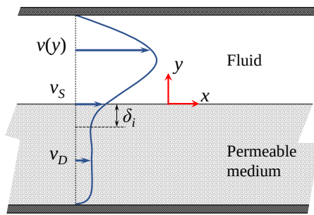
Figure 8.5: A typical velocity profile in a channel flow with a permeable medium layer.
