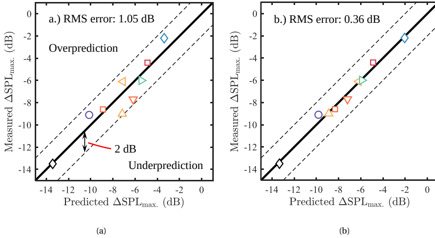
Figure 7.10: Prediction accuracy of the selected individuals in the Pareto front of the symbolic regression modeling trial 3.
