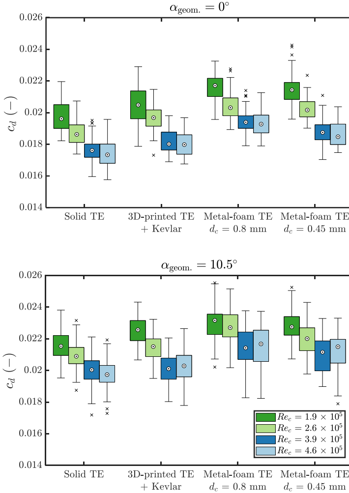
Figure 6.15: Drag coefficients of the NACA 0018 airfoil with various TE inserts for four different chord-based Reynolds number and geometrical angles of attack of 0^\circ (upper) and 10.5^\circ (lower).
