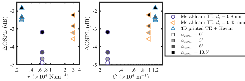
Figure 6.8: Noise attenuation of the airfoil with various permeable TE inserts at the chord-based Reynolds number of Re_c = 4.6 \times 10^5 and various geometrical angles of attack as functions of the flow resistivity (left) and form drag coefficient (right).
