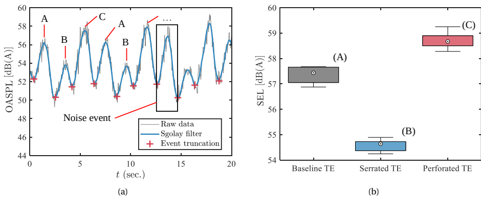
Figure 8.2: (a) Time-series OASPL data of 20-second recording from the Prototype 6 wind turbine where the three blades are treated differently and (b) SEL given by each blade of the Prototype 6 wind turbine.
