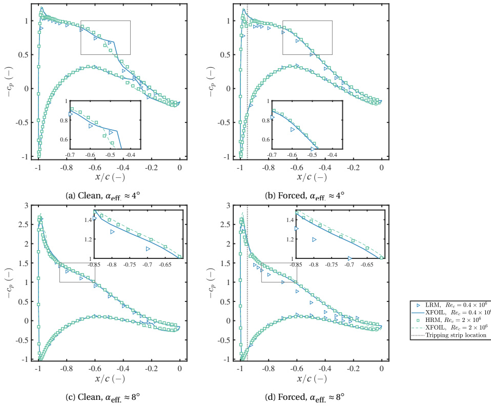
Figure 5.6: Comparison of c_p distributions from the A-Tunnel and the LTT tests of the baseline NACA 633-018 airfoil at various Re_c and non-zero \alpha_{\text{eff}} .
