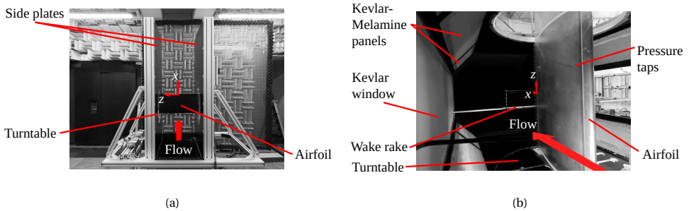
Figure 3.4: NACA 633-018 airfoil models installed in (a) the A-Tunnel and (b) the LTT.
