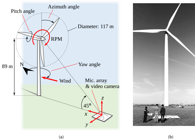
Figure 1.4: Wind turbine noise measurement set up: (a) A schematic (not to scale) and (b) a photograph.
