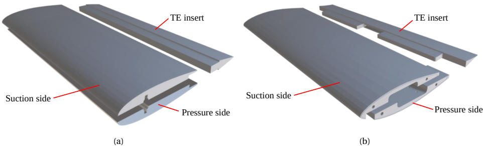
Figure 3.2: Components of the airfoil models for the A-Tunnel tests (a) NACA 0018 (b) NACA 633-018.
