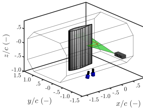
Figure 3.5: Schematics of the PIV set up used for characterizing the boundary layer properties over the NACA 633-018 airfoil model in the LTT.
