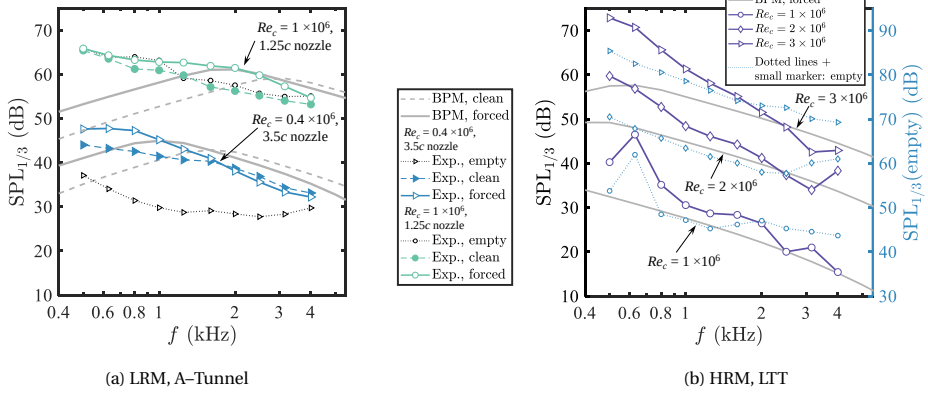
Figure 5.9: SPL spectra for the airfoils with baseline TE at various Re_c and \alpha_{\text{eff.}} \approx 0^\circ considering natural and forced transition configurations compared to the background flow noise levels and the BPM model. The different Re_c and facilities are annotated in the plots.
