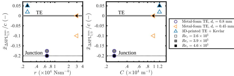
Figure 6.13: Streamwise locations of the maximum \Delta\text{SPL} given by various permeable TE inserts at various chord-based Reynolds numbers at zero-degree geometrical angle of attack as functions of the flow resistivity (left) and form drag coefficient (right).
