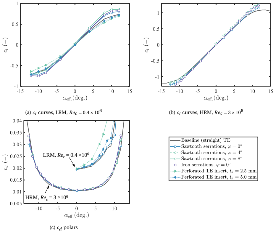
Figure 5.12: Measured aerodynamic coefficients with different TE add-ons installed. Only the forced transition location configuration is considered.
