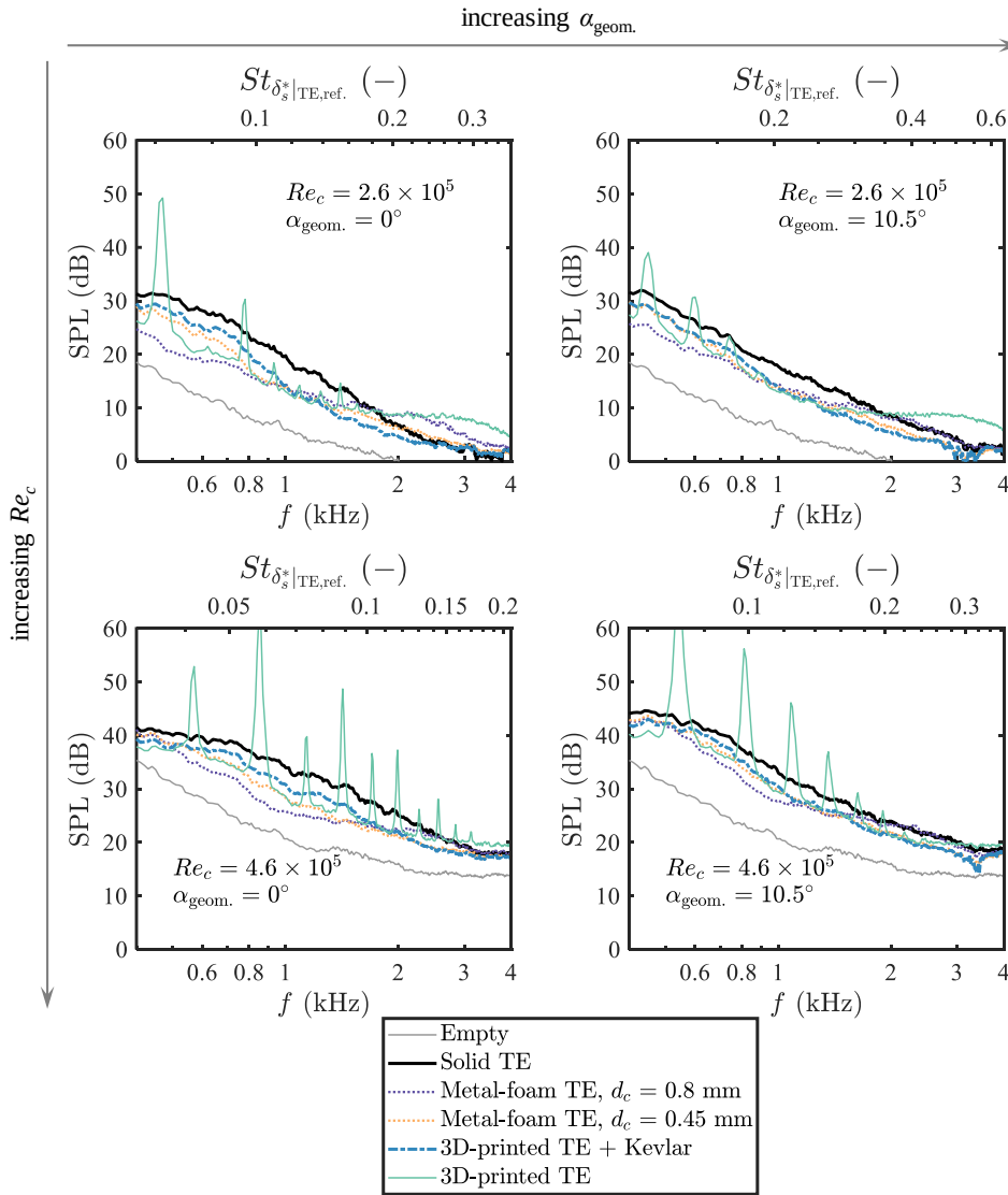
Figure 6.3: Narrow-band SPL spectra of the NACA 0018 airfoil with various permeable TE inserts at different given combinations of chord-based Reynolds numbers and geometrical angles of attack, compared to the reference solid TE insert and empty test section background noise.
