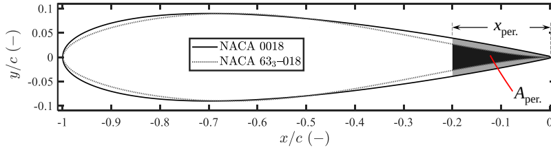
Figure 7.1: Airfoil profiles with a permeable TE insert considered.
