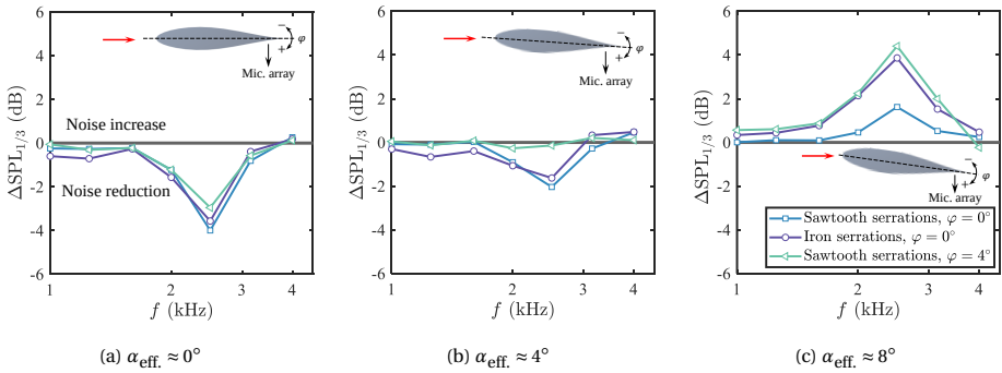
Figure 5.16: One-third octave band sound pressure level noise reduction spectra for the HRM under forced transition condition with serrated TEs at Re_c = 2 \times 10^6 and various \alpha_{eff} .
