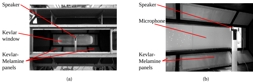
Figure B.1: Set up of the speaker and microphone in the empty LTT test section (a) viewed from outside of the test section and (b) viewed from inside of the test section.
