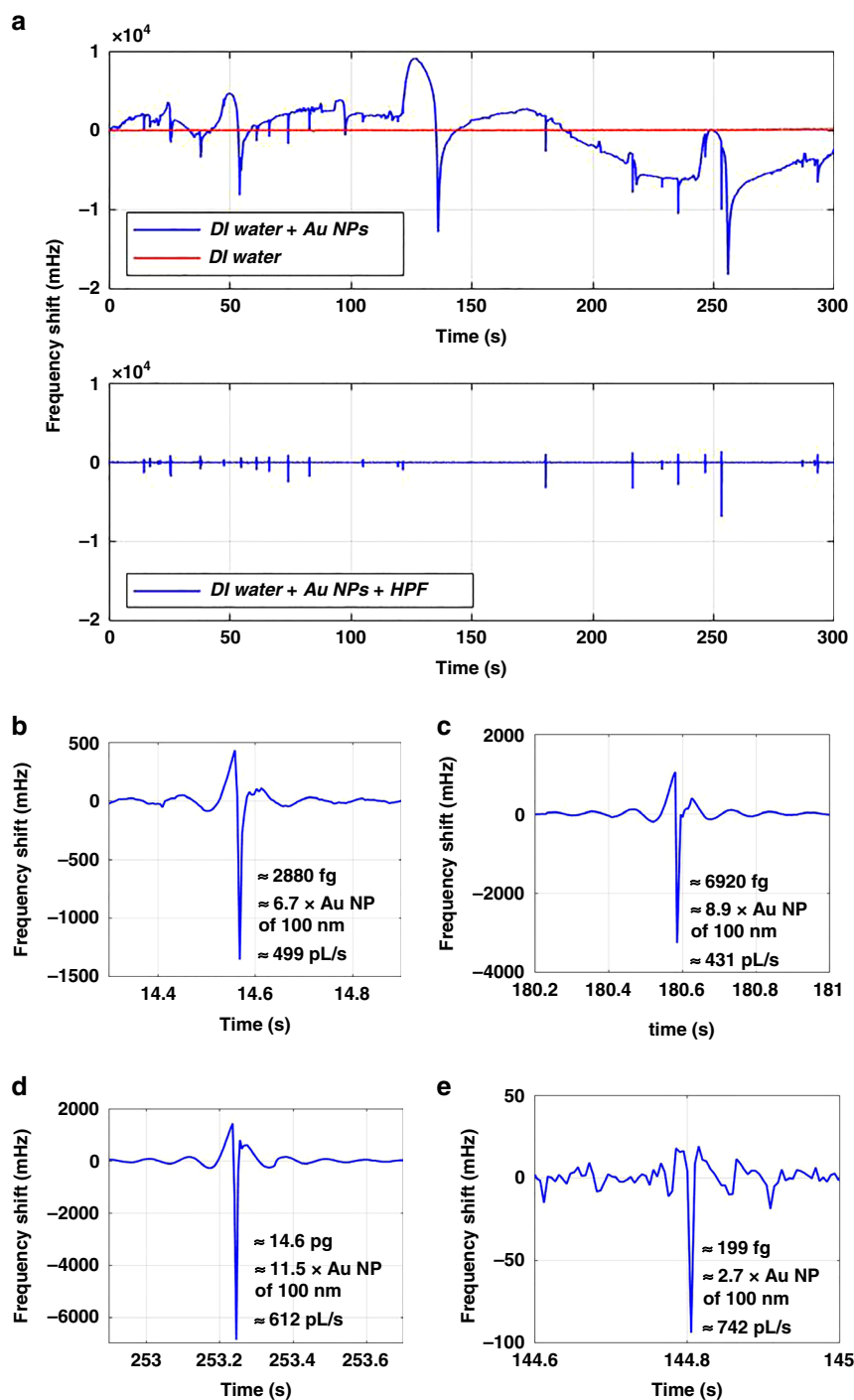
Fig. 6 Real-time mass detection of particles as they flow through the channel. a (Upper panel) Comparison of frequency shifts when DI water was flowing with an applied pressure difference of 70 mbar (red), and when a solution of 100 nm diameter gold nanoparticles was flowing with an applied pressure difference of 500 mbar (blue). (Lower panel) The data obtained after applying a high-pass filter with a cut-off frequency of 10 Hz on the data with nanoparticles flowing through the channel (blue curve in the upper panel). b–e Zoom-in views from a corresponding to particle detection events. The calculated masses and their equivalent Au particle's diameters are shown, along with the flow rates, estimated from the particle transient time
