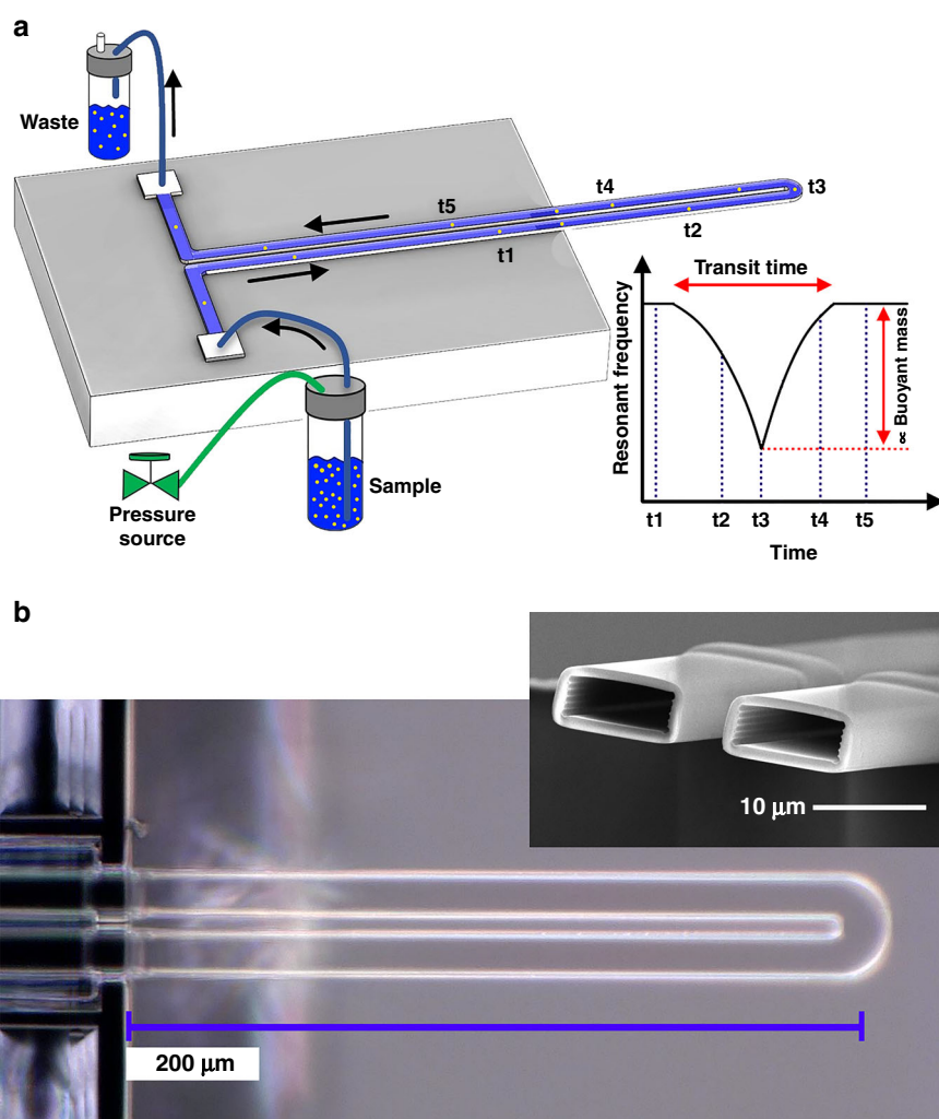
Fig. 1 Experimental schematic and device description. a Schematic of the experimental setup to determine the buoyant mass of nanoparticles using a cantilever-shaped suspended microchannel resonator (SMR). Particles flow through the channel from the sample reservoir (inlet) to the waste reservoir (outlet). The time points t1 to t5 represent the position of the nanoparticle as it flows through the channel. The plot shows a representative resonant frequency shift with time for the fundamental resonant mode. b Optical microscope top-view image of the U-shaped silicon dioxide SMR. A scanning electron microscope image of the cantilever cross-section is shown in the inset
