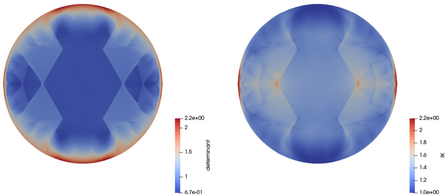
Fig. 9 Compatible deformation \hat{\varphi} from \|\nabla\varphi - \hat{P}\|_{L^2(\Omega)} \rightarrow \min for the matrix field \hat{P} shown in the Fig. 8. Colors show determinant (left) and the distortion \mathbb{K}(\nabla\hat{\varphi}) = \frac{1}{2} \frac{\|\nabla\hat{\varphi}\|^2}{\det \nabla\hat{\varphi}} (right) (Color figure online)
