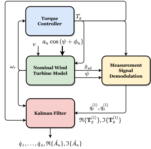
Fig. 3. Implementation of the proposed KF based on the demodulated wind turbine and tower model. The KF estimates the demodulated periodic load components, as well as the unmeasurable tower states, and takes inputs from the torque controller and the (MSD-demodulated) nominal wind turbine model measurements.
