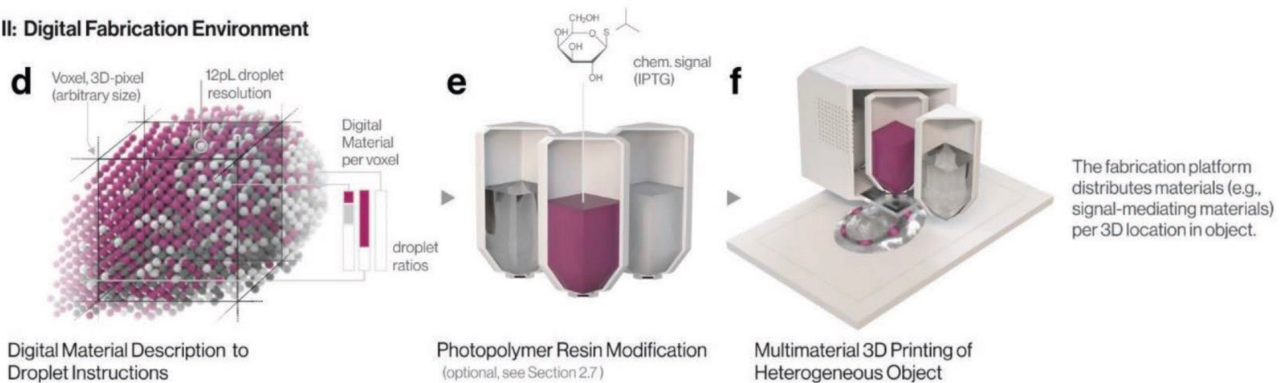
Figure 4. Scaffold fabrication process of Vespers III.
