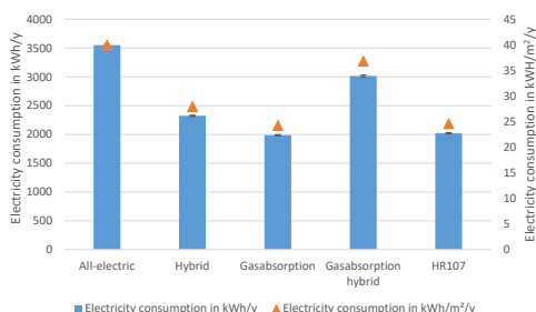
FIG. 4.3 Average electricity consumption per dwelling and per m 2 to heat pump type
