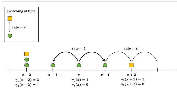
Figure 5.1: Representation via slow and fast particles moving on the one-layer graph \mathbb{Z} ( \sigma = 0 ).
