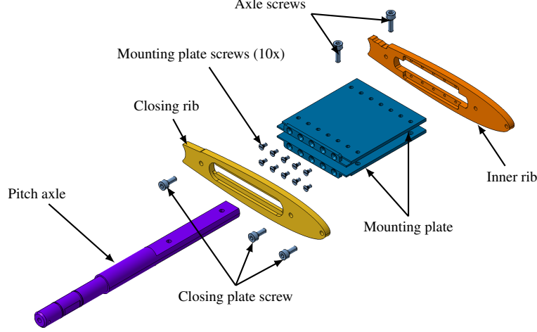
Figure 6: Exploded view of the right-hand side mounting.
