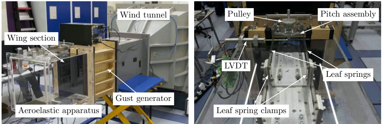
(a) Wind tunnel with the gust generator and aeroelastic apparatus.
