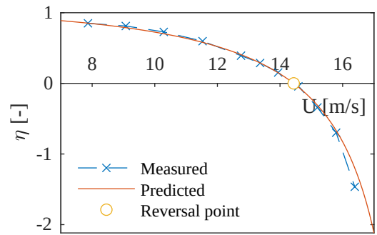
Figure 13: Theoretical and measured control surface efficiency versus velocity.
