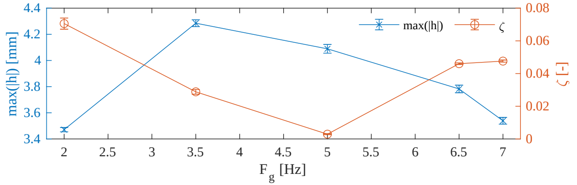
Figure 19: Comparison of the open-loop maximum amplitude and damping coefficient versus gust frequency.
