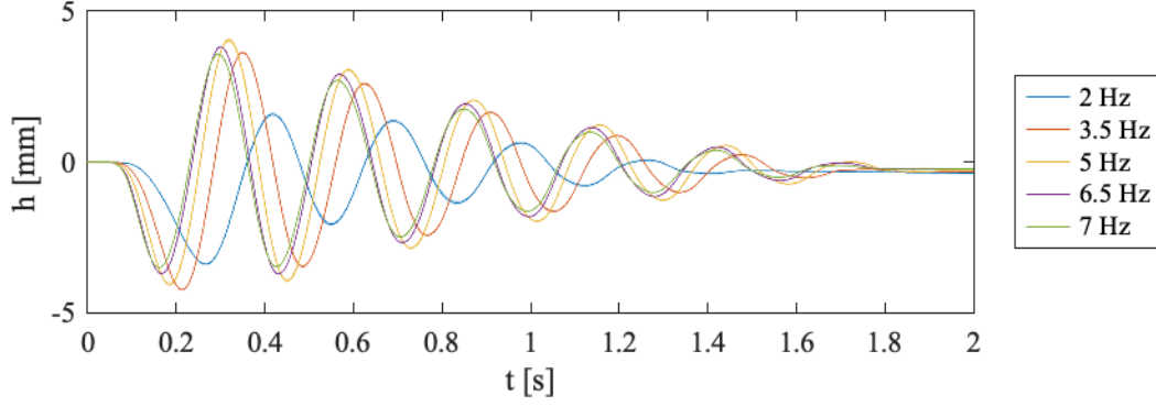
Figure 18: The open-loop heave response for increasing gust frequencies.
