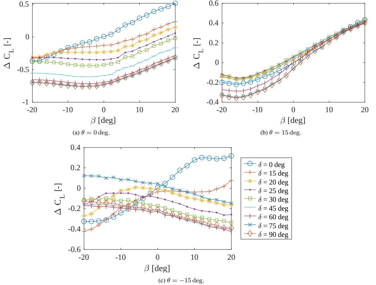
Figure 16: \Delta C_L - \beta curves for varying \delta , Re = 1.245 \times 10^5 .
