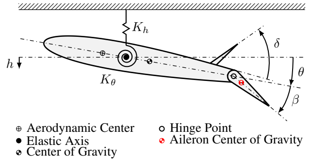
Figure 1: Schematic of the wing section and sign conventions.
