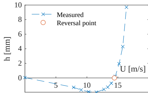
Figure 12: Heave response to a 20 deg aileron deflection versus velocity. Control reversal occurs at U = 14.4 m/s.
