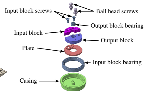
Figure 5: Exploded view of the freeplay mechanism.
