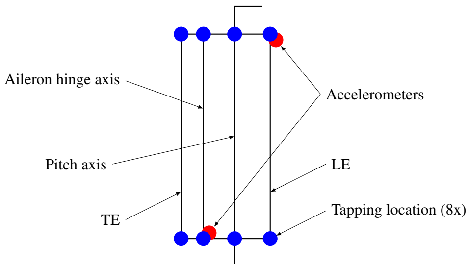
Figure 9: Schematic of the GVT wing model.
