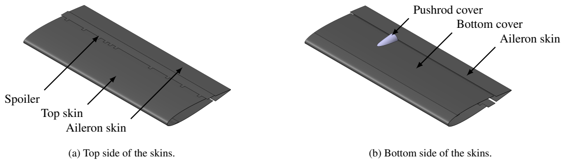
Figure 3: Renders of the wing skins.
