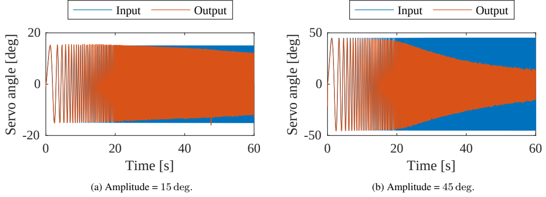
Figure 14: Servo response to a chirp signal from 0.1 Hz to 10 Hz.
