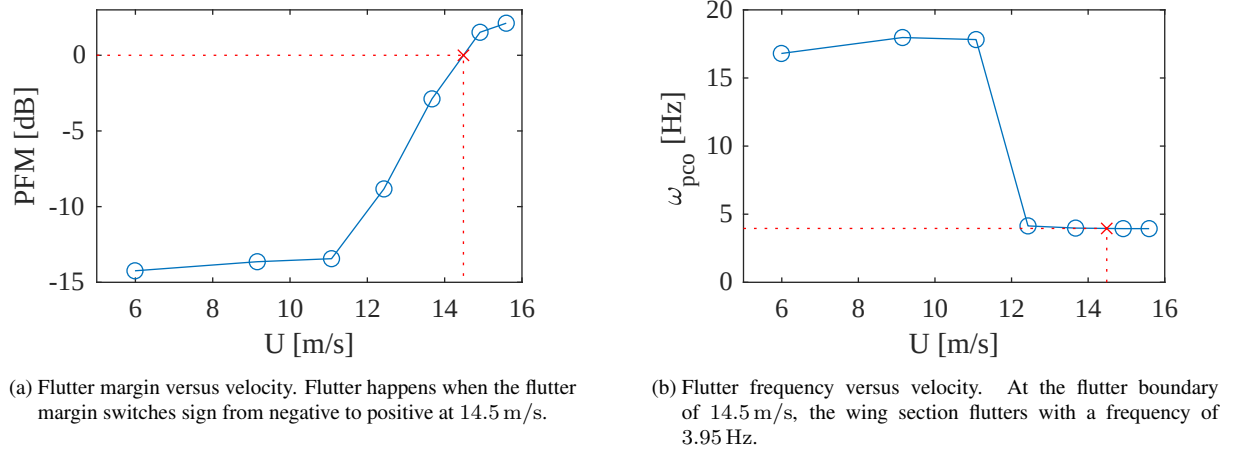
Figure 11: Parametric flutter margin results.
