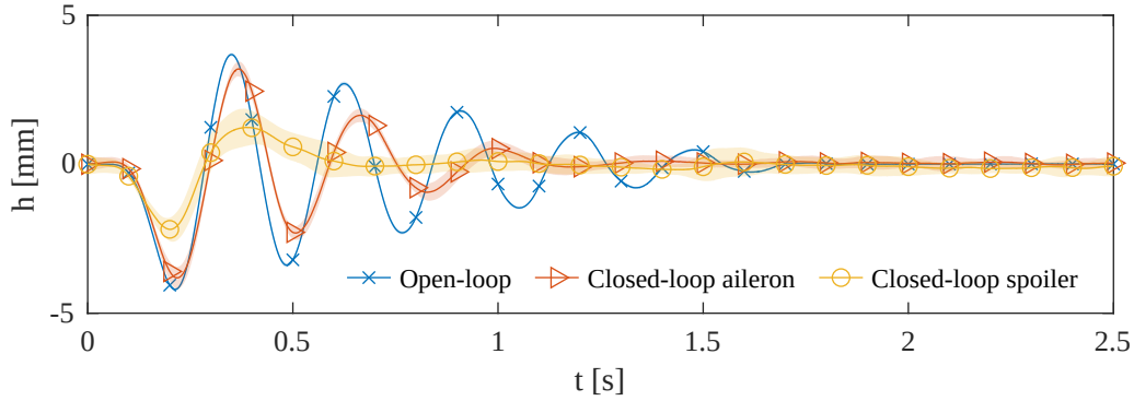
Figure 20: Comparison of the open-loop and closed-loop gust responses.
