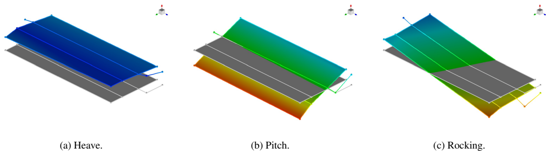
Figure 10: The first three structural modes.
