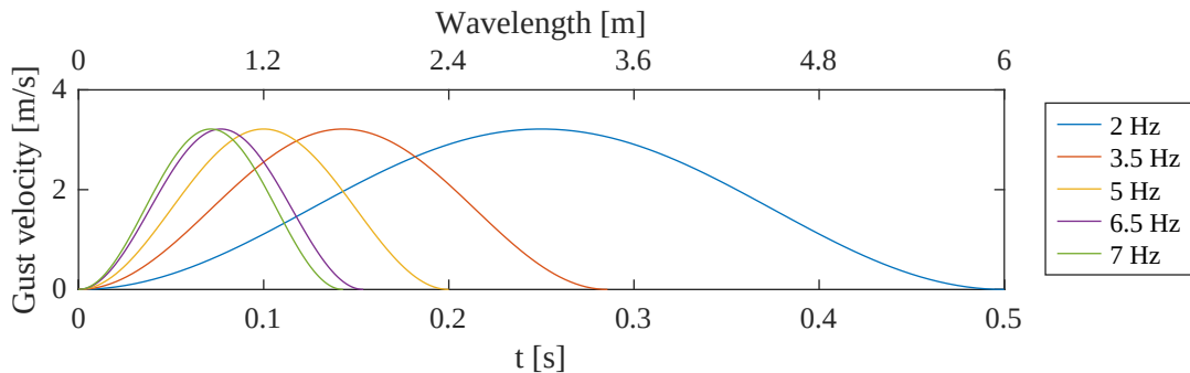
Figure 17: Gust profiles for gust frequencies of 2 Hz, 3.5 Hz, 5 Hz, 6.5 Hz, and 7 Hz at U = 13.6 m/s.
