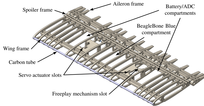
Figure 2: Render of the wing, spoiler and aileron frames.
