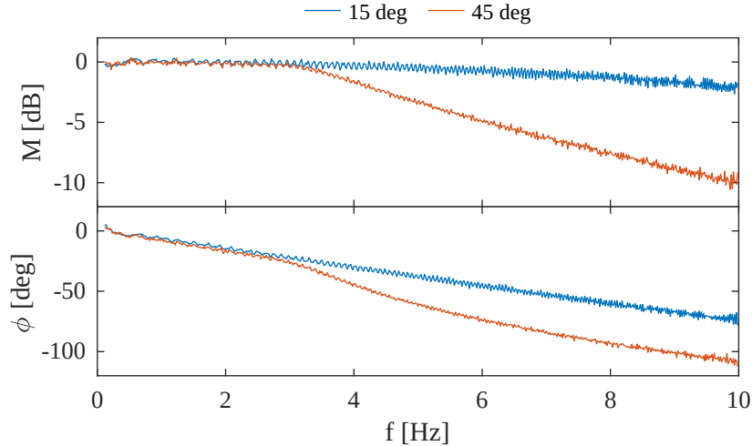
Figure 15: Bode plot of the servo actuator response.
