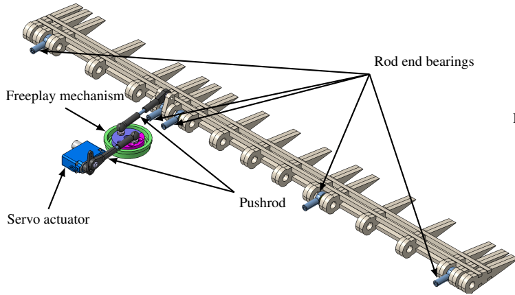
Figure 4: Render of the aileron actuation mechanism.
