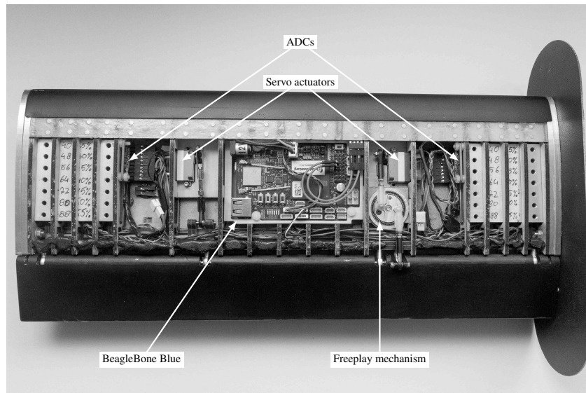
Figure 7: Bottom view of the wing section with the cover and right endplate removed.
