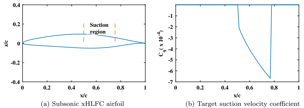
Fig. 17 Optimized airfoil shape and suction velocity coefficient
