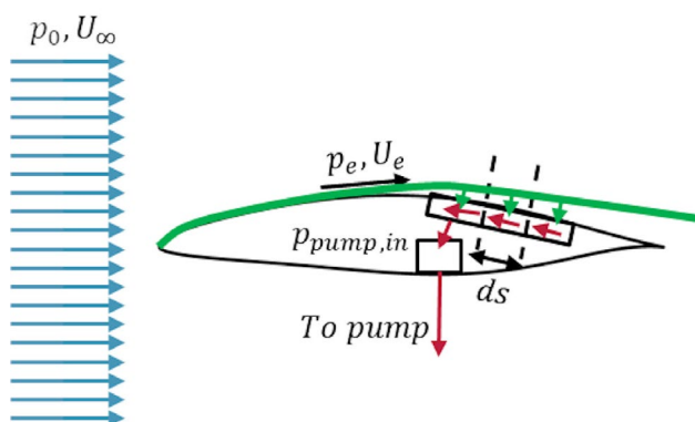
(a) Airflow path in xHLFC suction system
