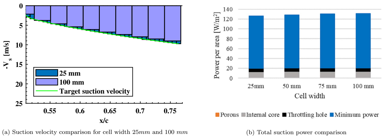
Fig. 25 Effect of internal core cell width on suction velocity and power
