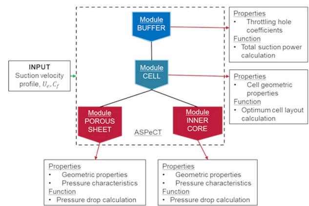
Fig. 5 Flowchart of ASPeCT
