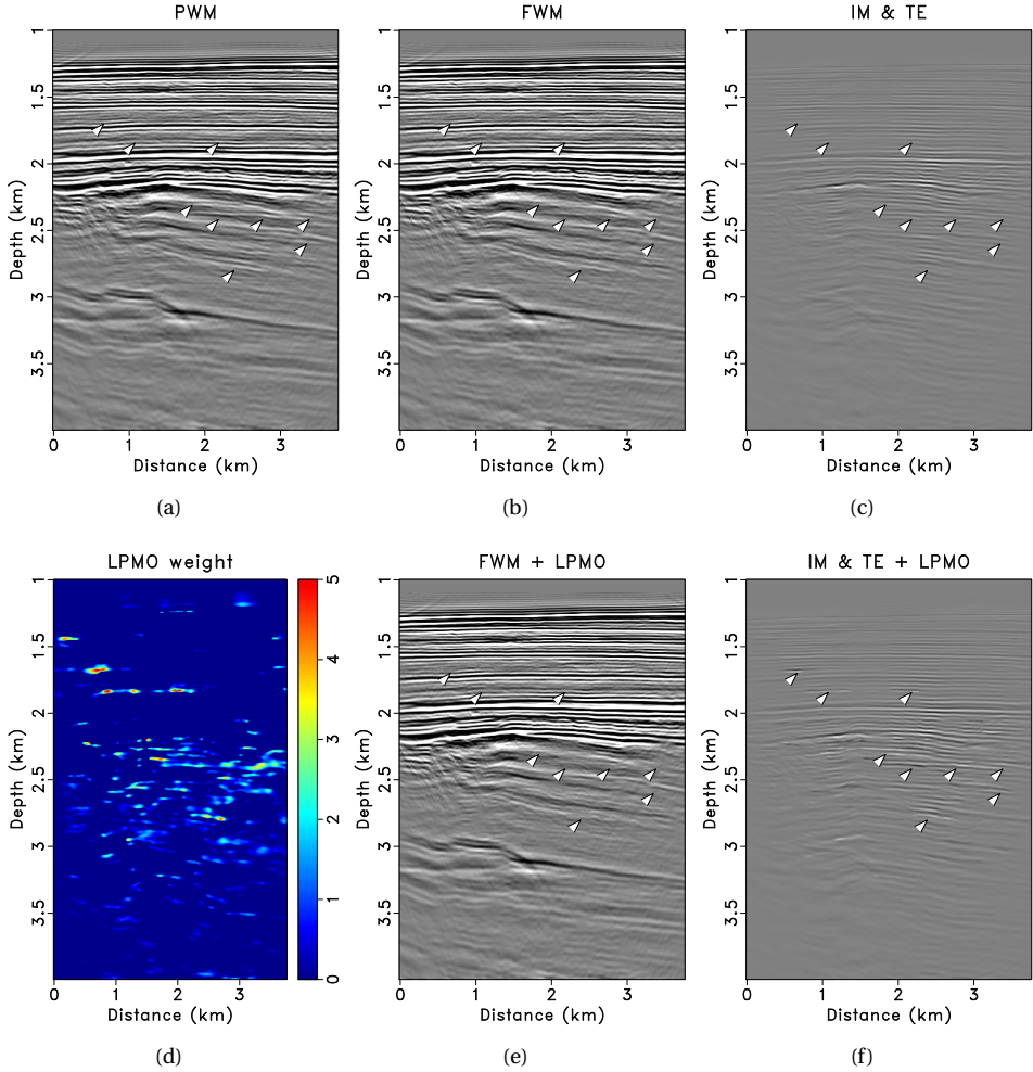
Figure A.1: LPMO on the FWM image of the Vøring field data set. (a) PWM image. (b) FWM image. (c) Difference image between PWM and FWM that includes the initially estimated internal multiples (IM) and transmission effects (TE). (d) Estimated positive-only LPMO weight related to the leaked internal multiple crosstalk in the FWM image. (e) Final estimated FWM image after LPMO. (f) Difference image that includes the final estimated internal multiples and transmission effects after LPMO.
