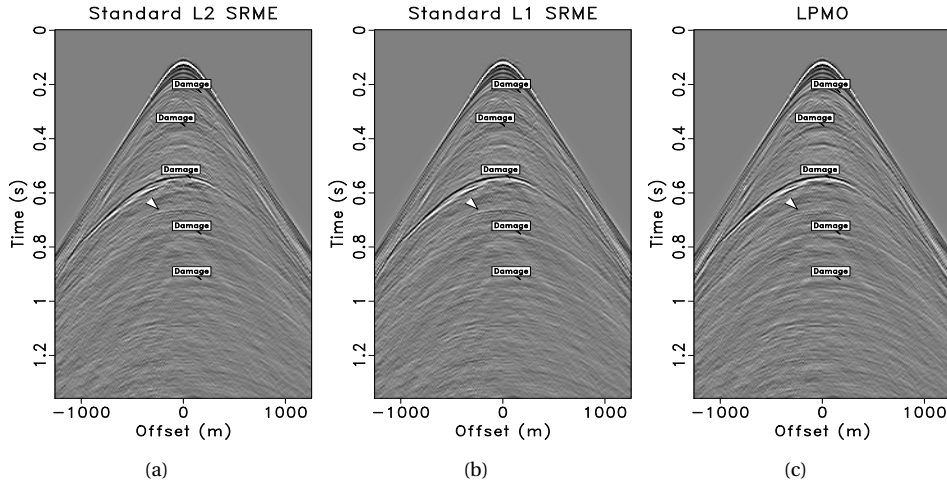
Figure 4.19: Shot gather comparison with the standard SRME. (a) L2-norm standard SRME primaries with 160 ms * 25 traces local subtraction window size. (b) L1-norm standard SRME primaries with 160 ms * 25 traces local subtraction window size. (c) The proposed primaries after LPMO (for comparison purpose). The arrows in (a) and (b) denote the more severe multiple leakage compared to (c). The rectangles in (a) and (b) denote more primary damage compared to (c).
