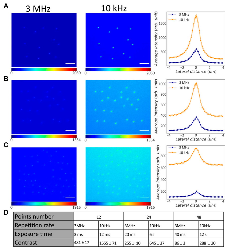
FIGURE 3 Comparison between point-cloud CGHs projected into liquid fluorescein with different repetition rates. (A) Left: TPEF image of 12-point CGH projected with 3 MHz repetition rate. Middle: TPEF image of the same CGH projected with 10 kHz repetition rate. Scale bar: 25 \mu\text{m} . Right: Average line profiles across the pixel of maximum intensity for all the points projected with 3 MHz (blue rhombuses) and 10 kHz (orange dots) repetition rate. Continuous lines: Lorentzian fit on the data points; shadow areas: s.e.m.; orange: 10 kHz; blue: 3 MHz. (B) Left: TPEF image of 24-point CGH projected with 3 MHz repetition rate. Middle: TPEF image of the same CGH projected with 10 kHz repetition rate. Right: Average line profiles across the pixel of maximum intensity for all the points projected with 3 MHz (blue rhombuses) and 10 kHz (orange dots) repetition rate. Continuous lines: Lorentzian fit on the data points; shadow areas: s.e.m.; orange: 10 kHz; blue: 3 MHz. (C) Left: TPEF image of 48-point CGH projected with 3 MHz repetition rate. Middle: TPEF image of the same CGH projected with 10 kHz repetition rate. Right: Average line profiles across the pixel of maximum intensity for all the points projected with 3 MHz (blue rhombuses) and 10 kHz (orange dots) repetition rate. Continuous lines: Lorentzian fit on the data points; shadow areas: s.e.m.; orange: 10 kHz; blue: 3 MHz. (D) Table with experimental parameters used to acquire each grid image, contrast and corresponding s.e.m.
