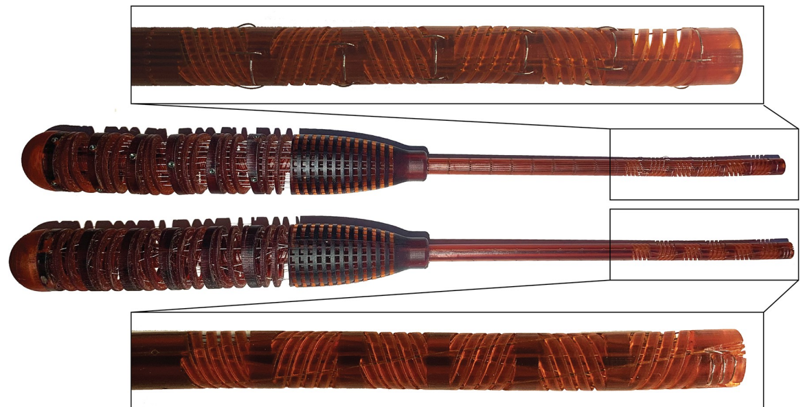
Fig 6. Instrument prototypes employing the parallel configuration (top) and multi configuration (bottom). The close-ups show the steerable shafts. Notice that the fixation points in the shafts differ, depending on the configuration. In the parallel configuration, each segment has two fixation points whereas in the multi configuration all cables are fixed at the distal end of the shaft.
