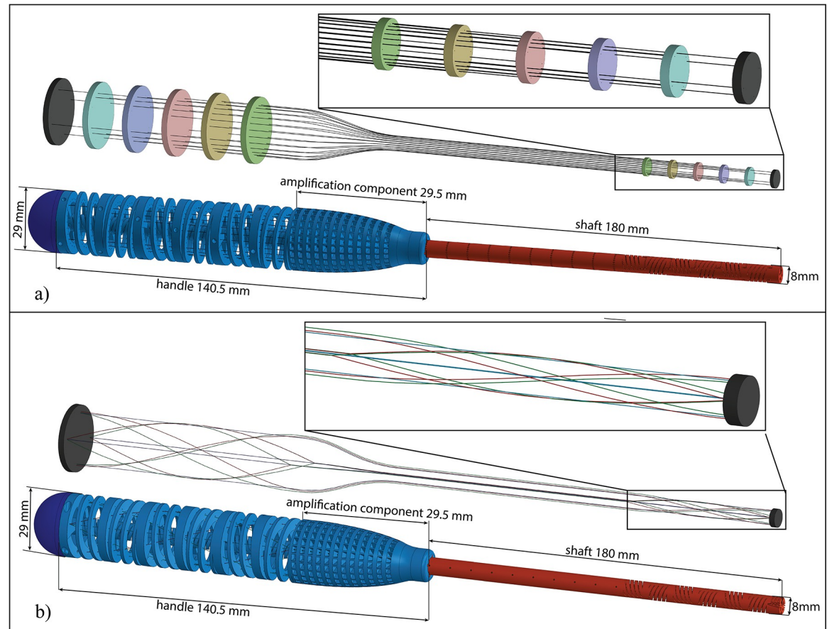
Fig 3. 3D model of the parallel and multi configurations. a) The parallel cable configuration with a close-up on the shaft and the final design of the device. Each color corresponds to a segment mirrored on the control side. b) Multi configuration of the cables and the final design of the device. In this configuration, all cables are connected at the ends. The close-up shows the cable configuration in the steerable shaft.
