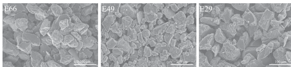
Figure 9. Scanning electron microscopy ( SEM ) images of sediment mixtures E29, E49, and E66.
