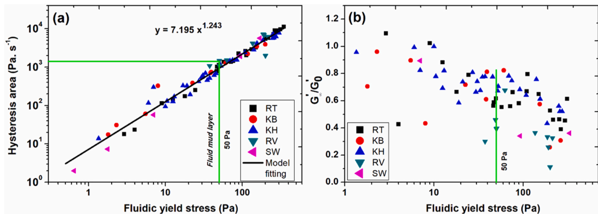
Fig. 7. (a) Hysteresis area (obtained from the time-dependent test) as a function of fluidic yield stress for different locations, (b) equilibrium structural parameter ( G'_\infty/G'_0 ) as a function of fluidic yield stress for different locations. Green solid line represents the critical value of fluidic yield stress (50 Pa) and hysteresis area ( 1400 \text{ Pa s}^{-1} ) for the fluid mud characterisation. (For interpretation of the references to colour in this figure legend, the reader is referred to the Web version of this article.)
