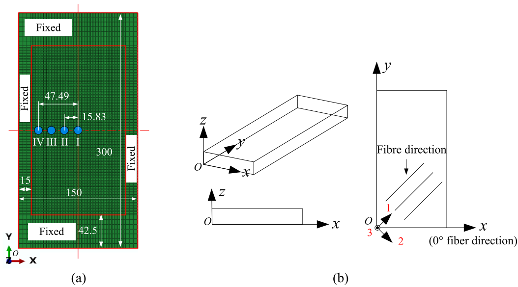
Fig. 1. (a) Panel dimensions of the FE model to calculate single central and eccentric indentation stress fields, (b) coordinate systems used in this study: global coordinate system (black x-y-z) and local coordinate system (red 1-2-3). (For interpretation of the references to colour in this figure legend, the reader is referred to the web version of this article.)
