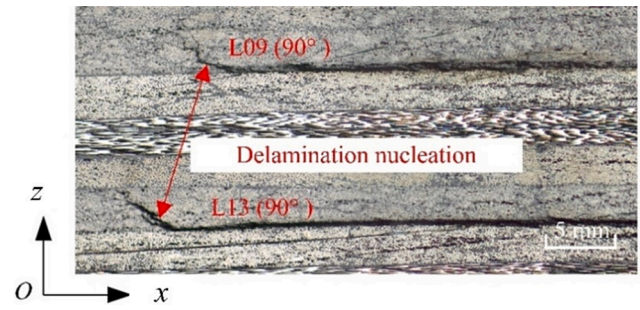
Fig. 6. Typical feature of the indentation delamination nucleation: a 45° incline from the normal direction.
