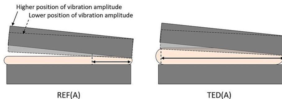
Fig. 9. Schematic of the wetting at the interface for cases REF(A) and TED(A). The double-arrow indicates the extend of ED volume that is in contact with the top adherend at some point during the vibration.
