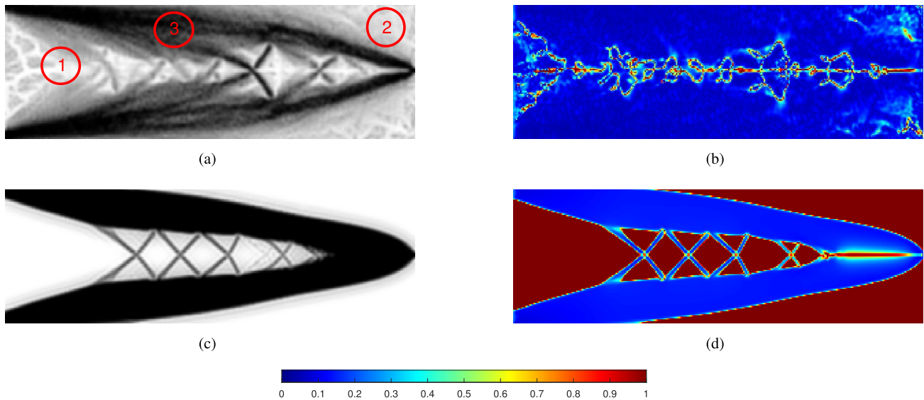
Fig. 8 Effect of threshold stress levels on intersection minimization results for Problem 1: a Design at 100 th iteration for \sigma_0 = 0 \text{ MPa} . b is the corresponding multi-axiality criterion 1/\log_2(H_e) . c and d Design and corresponding multi-axiality criteria at 100 th iteration for \sigma_0 = 10 \text{ MPa} . The threshold stress is selected from the refer-
