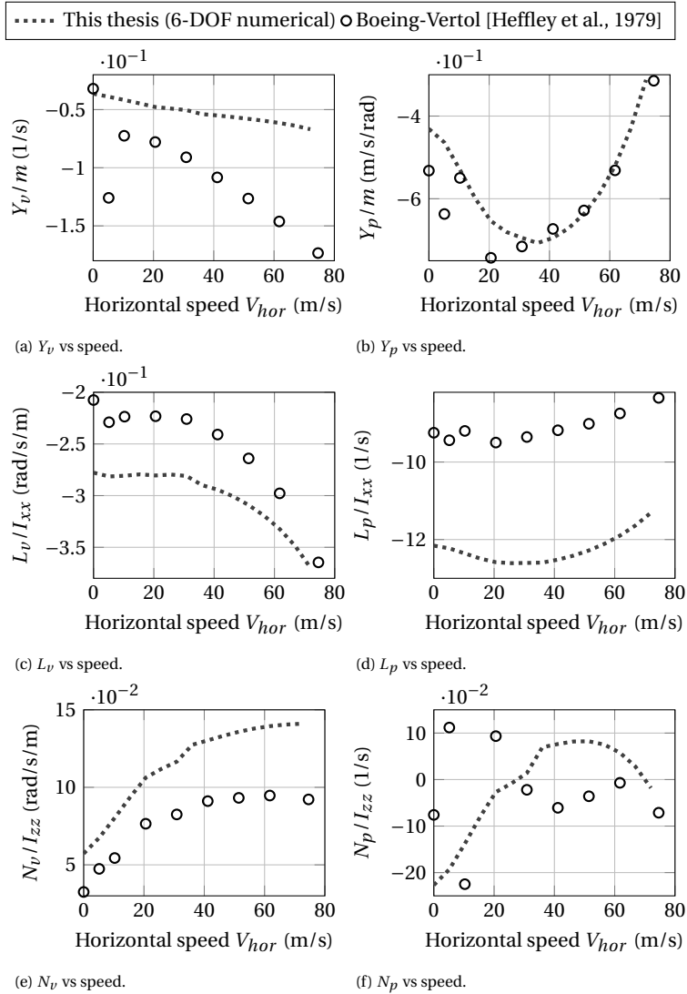
Figure C.2: Stability derivatives in straight level flight at sea-level (MTOW, \psi_{mr} = 100\% ) as a function of horizontal speed for the lateral-directional dynamics. ( Continues. )
